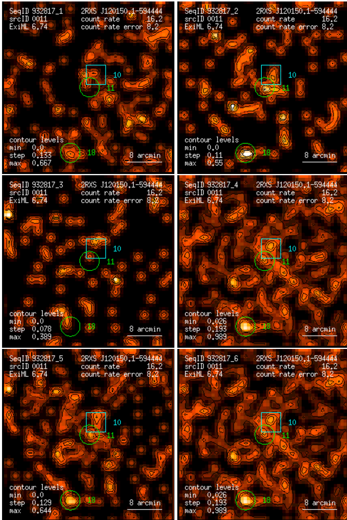
Figure 11: RASS 932817: detection 0011: band rate images, Gaussian filter: (1) PSPC channels 11 – 41, (2) 52 – 90, (3) 91 – 201, (4) 11 – 235, (5) 52 – 201, (6) 11 – 201. Broad band rates in counts/ks. Band rate contour levels in counts/ks/arcmin 2 .
