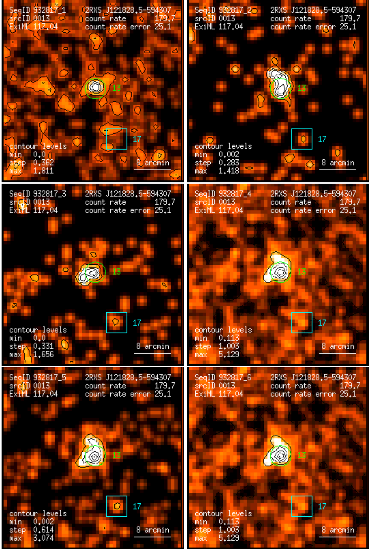
Figure 13: RASS 932817: detection 0013: band rate images, Gaussian filter: (1) PSPC channels 11 – 41, (2) 52 – 90, (3) 91 – 201, (4) 11 – 235, (5) 52 – 201, (6) 11 – 201. Broad band rates in counts/ks. Band rate contour levels in counts/ks/arcmin 2 .
