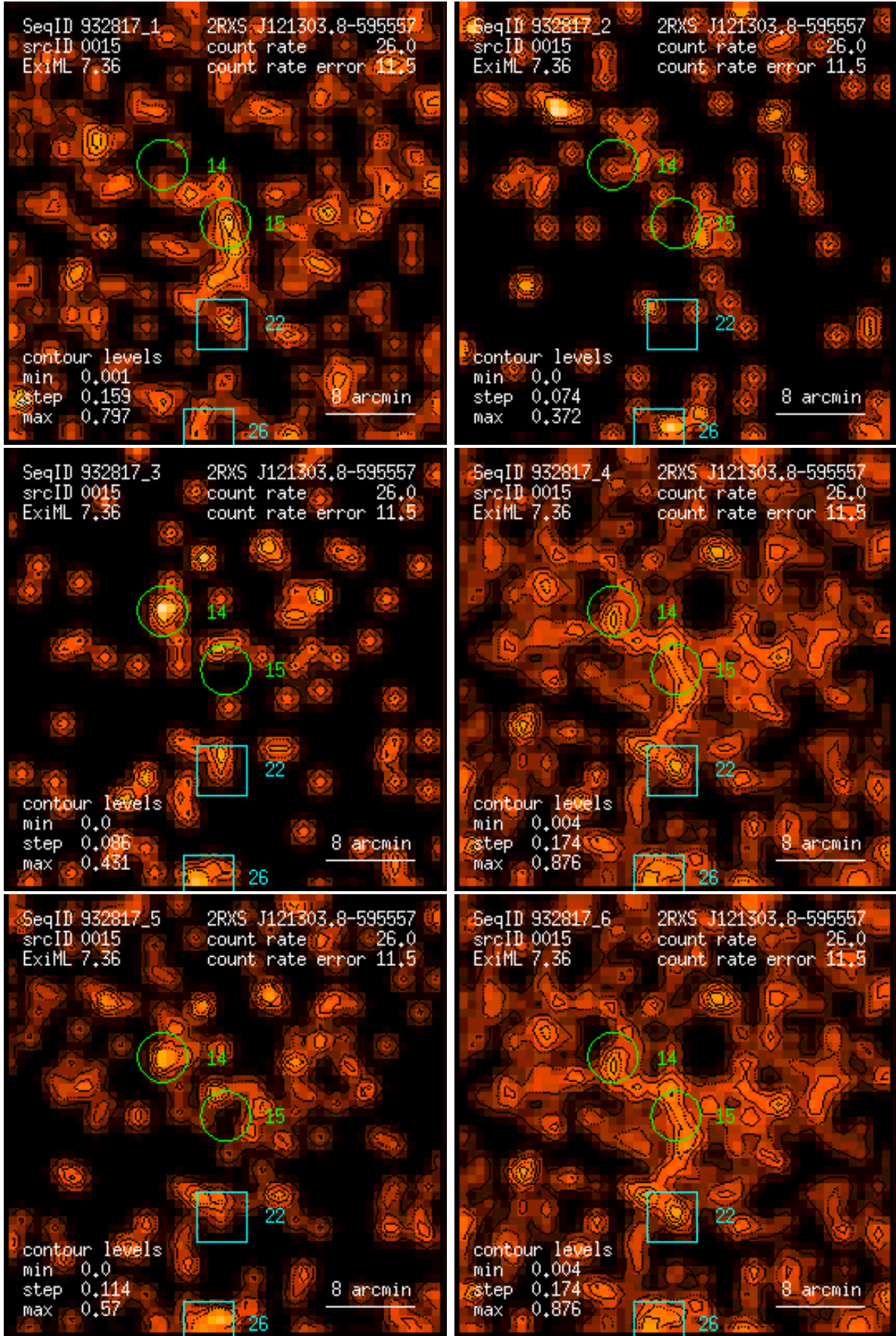
Figure 15: RASS 932817: detection 0015: band rate images, Gaussian filter: (1) PSPC channels 11 – 41, (2) 52 – 90, (3) 91 – 201, (4) 11 – 235, (5) 52 – 201, (6) 11 – 201. Broad band rates in counts/ks. Band rate contour levels in counts/ks/arcmin 2 .
