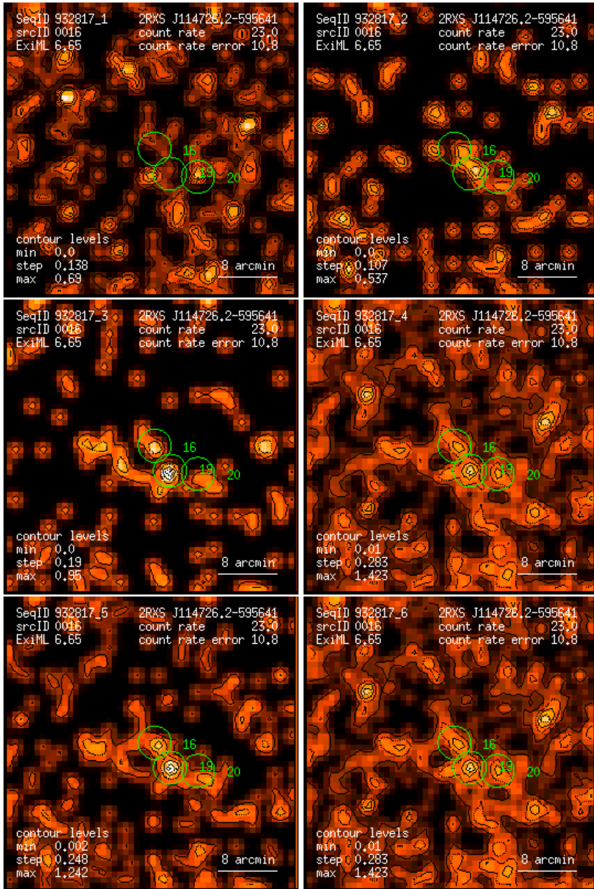
Figure 16: RASS 932817: detection 0016: band rate images, Gaussian filter: (1) PSPC channels 11 – 41, (2) 52 – 90, (3) 91 – 201, (4) 11 – 235, (5) 52 – 201, (6) 11 – 201. Broad band rates in counts/ks. Band rate contour levels in counts/ks/arcmin 2 .
