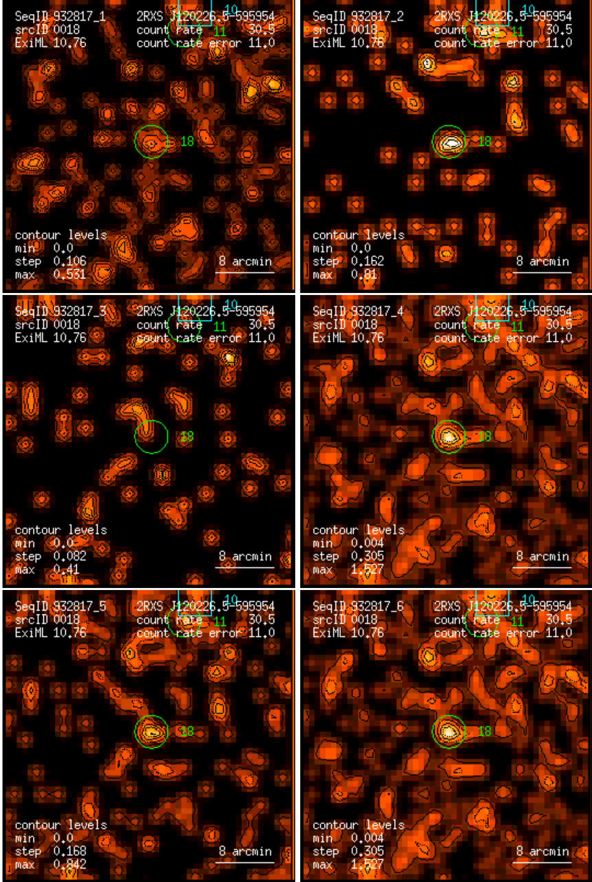
Figure 18: RASS 932817: detection 0018: band rate images, Gaussian filter: (1) PSPC channels 11 – 41, (2) 52 – 90, (3) 91 – 201, (4) 11 – 235, (5) 52 – 201, (6) 11 – 201. Broad band rates in counts/ks. Band rate contour levels in counts/ks/arcmin 2 .
