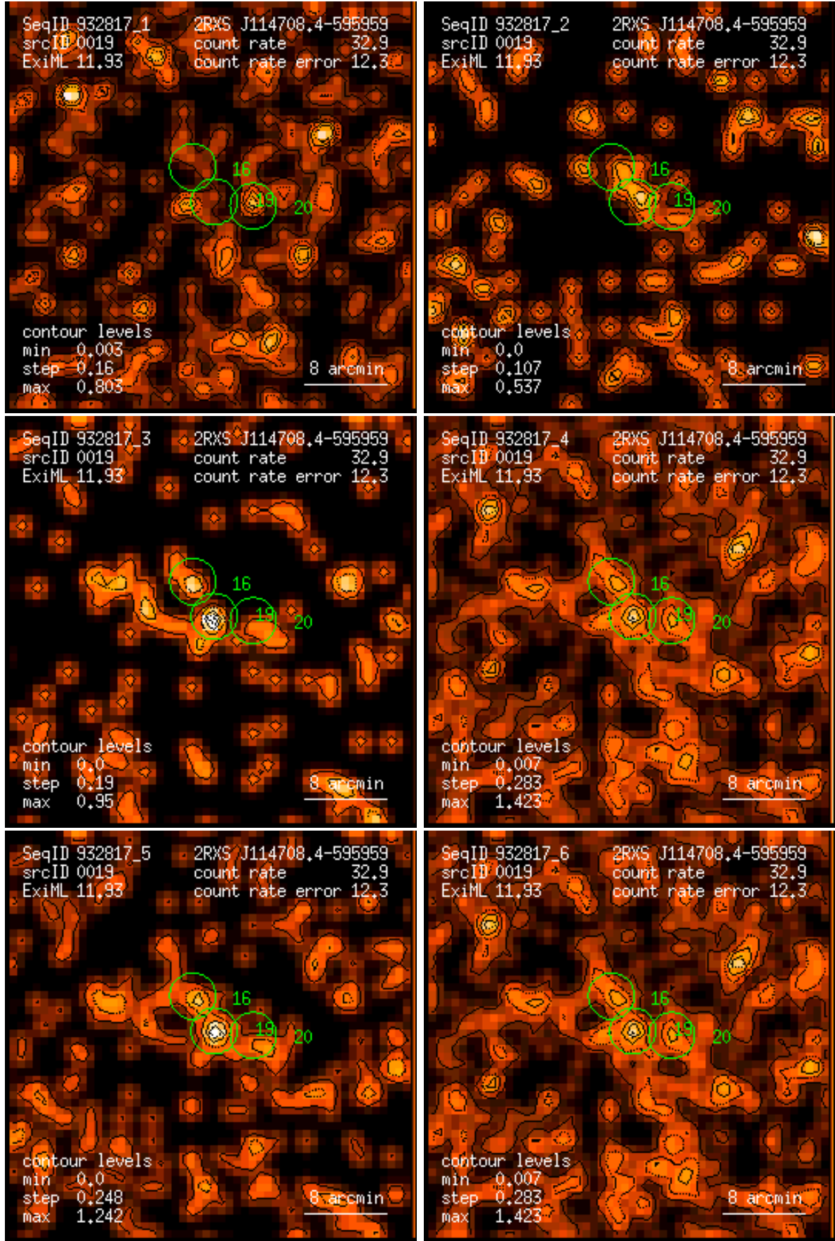
Figure 19: RASS 932817: detection 0019: band rate images, Gaussian filter: (1) PSPC channels 11 – 41, (2) 52 – 90, (3) 91 – 201, (4) 11 – 235, (5) 52 – 201, (6) 11 – 201. Broad band rates in counts/ks. Band rate contour levels in counts/ks/arcmin 2 .
