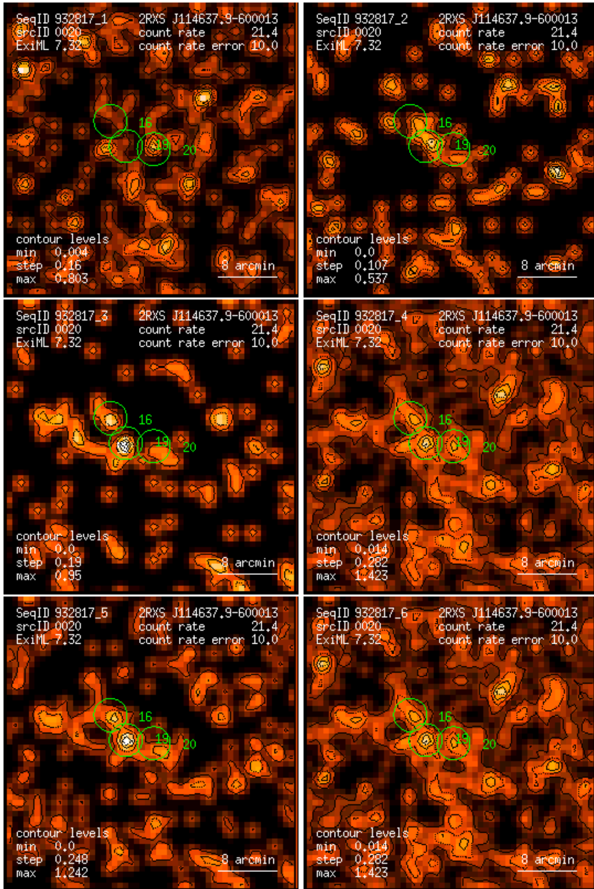
Figure 20: RASS 932817: detection 0020: band rate images, Gaussian filter: (1) PSPC channels 11 – 41, (2) 52 – 90, (3) 91 – 201, (4) 11 – 235, (5) 52 – 201, (6) 11 – 201. Broad band rates in counts/ks. Band rate contour levels in counts/ks/arcmin 2 .
