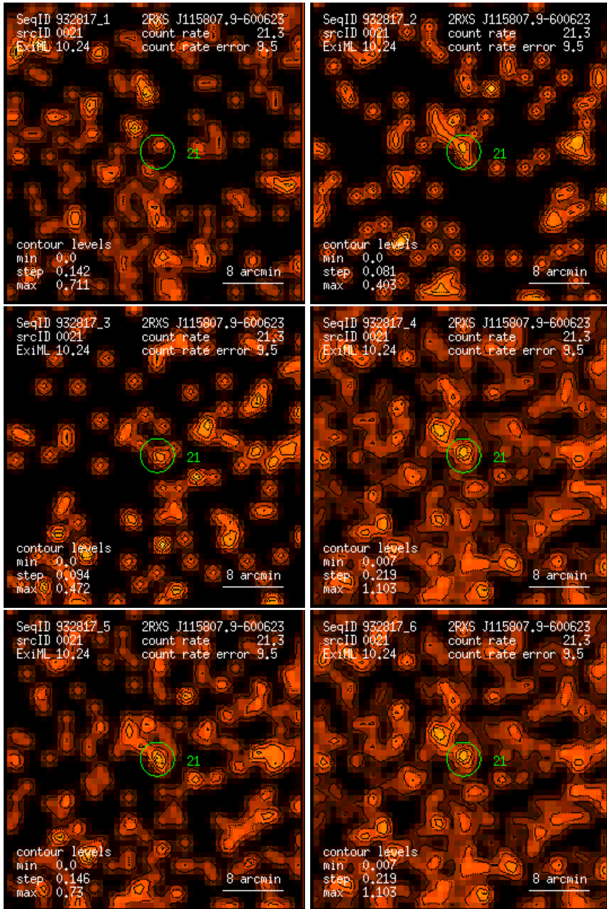
Figure 21: RASS 932817: detection 0021: band rate images, Gaussian filter: (1) PSPC channels 11 – 41, (2) 52 – 90, (3) 91 – 201, (4) 11 – 235, (5) 52 – 201, (6) 11 – 201. Broad band rates in counts/ks. Band rate contour levels in counts/ks/arcmin 2 .
