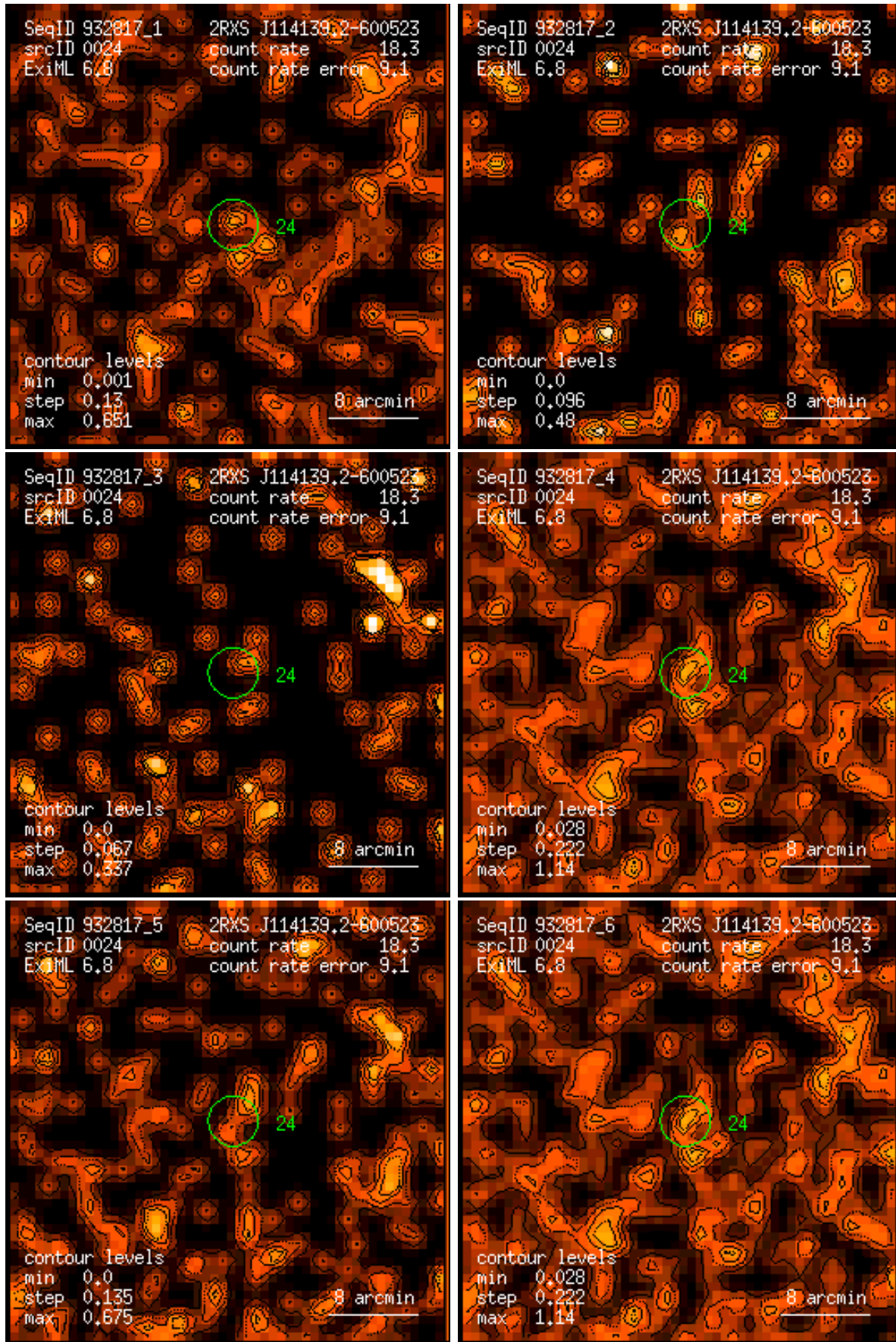
Figure 24: RASS 932817: detection 0024: band rate images, Gaussian filter: (1) PSPC channels 11 – 41, (2) 52 – 90, (3) 91 – 201, (4) 11 – 235, (5) 52 – 201, (6) 11 – 201. Broad band rates in counts/ks. Band rate contour levels in counts/ks/arcmin 2 .
