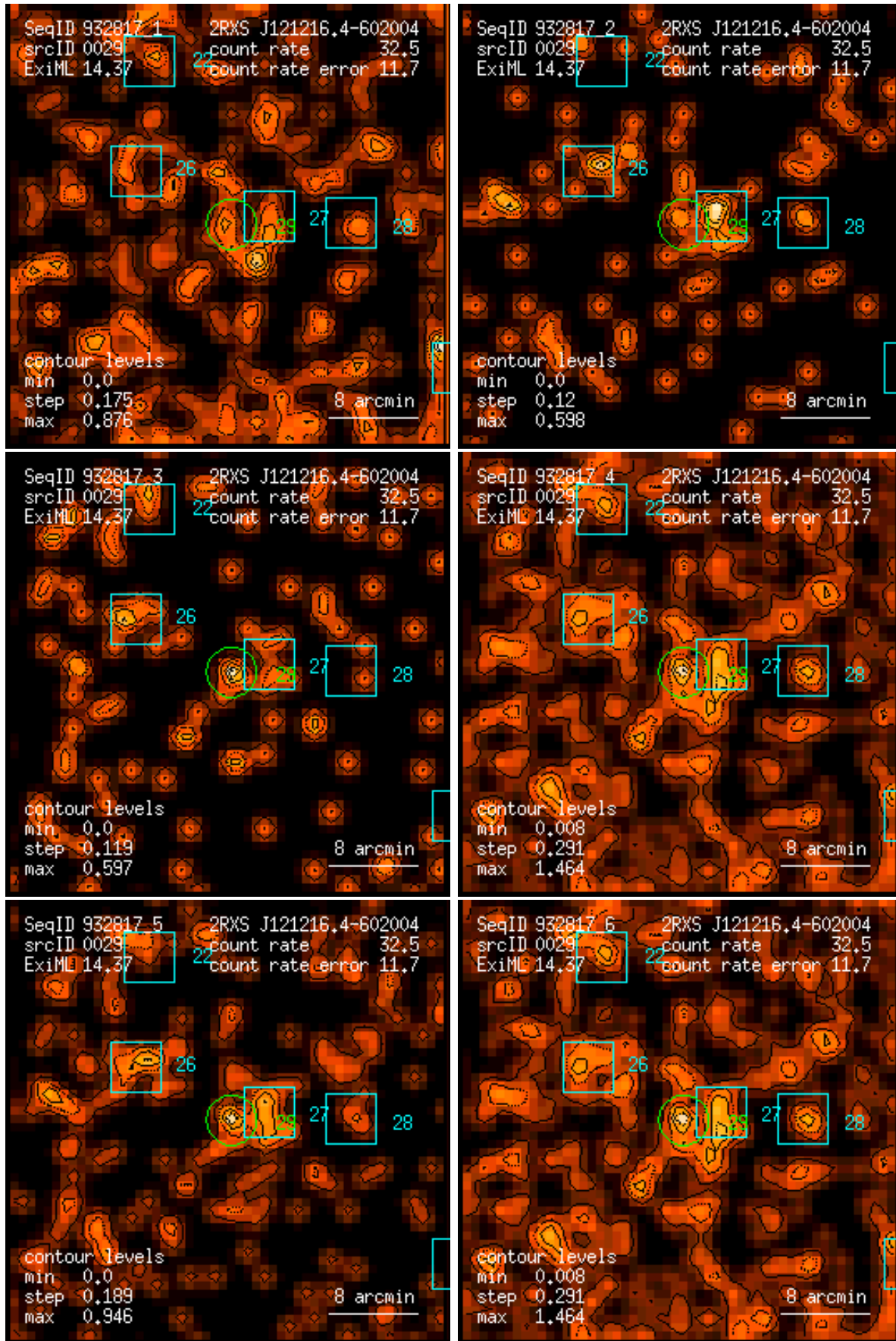
Figure 29: RASS 932817: detection 0029: band rate images, Gaussian filter: (1) PSPC channels 11 – 41, (2) 52 – 90, (3) 91 – 201, (4) 11 – 235, (5) 52 – 201, (6) 11 – 201. Broad band rates in counts/ks. Band rate contour levels in counts/ks/arcmin 2 .
