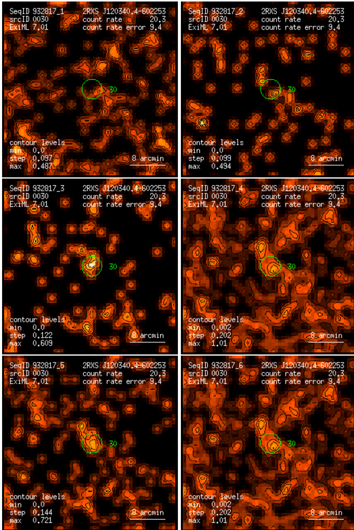
Figure 30: RASS 932817: detection 0030: band rate images, Gaussian filter: (1) PSPC channels 11 – 41, (2) 52 – 90, (3) 91 – 201, (4) 11 – 235, (5) 52 – 201, (6) 11 – 201. Broad band rates in counts/ks. Band rate contour levels in counts/ks/arcmin 2 .
