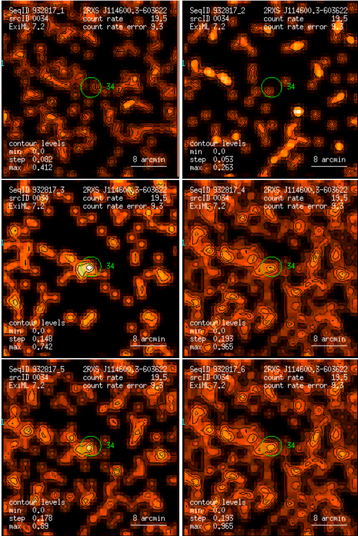
Figure 34: RASS 932817: detection 0034: band rate images, Gaussian filter: (1) PSPC channels 11 – 41, (2) 52 – 90, (3) 91 – 201, (4) 11 – 235, (5) 52 – 201, (6) 11 – 201. Broad band rates in counts/ks. Band rate contour levels in counts/ks/arcmin 2 .
