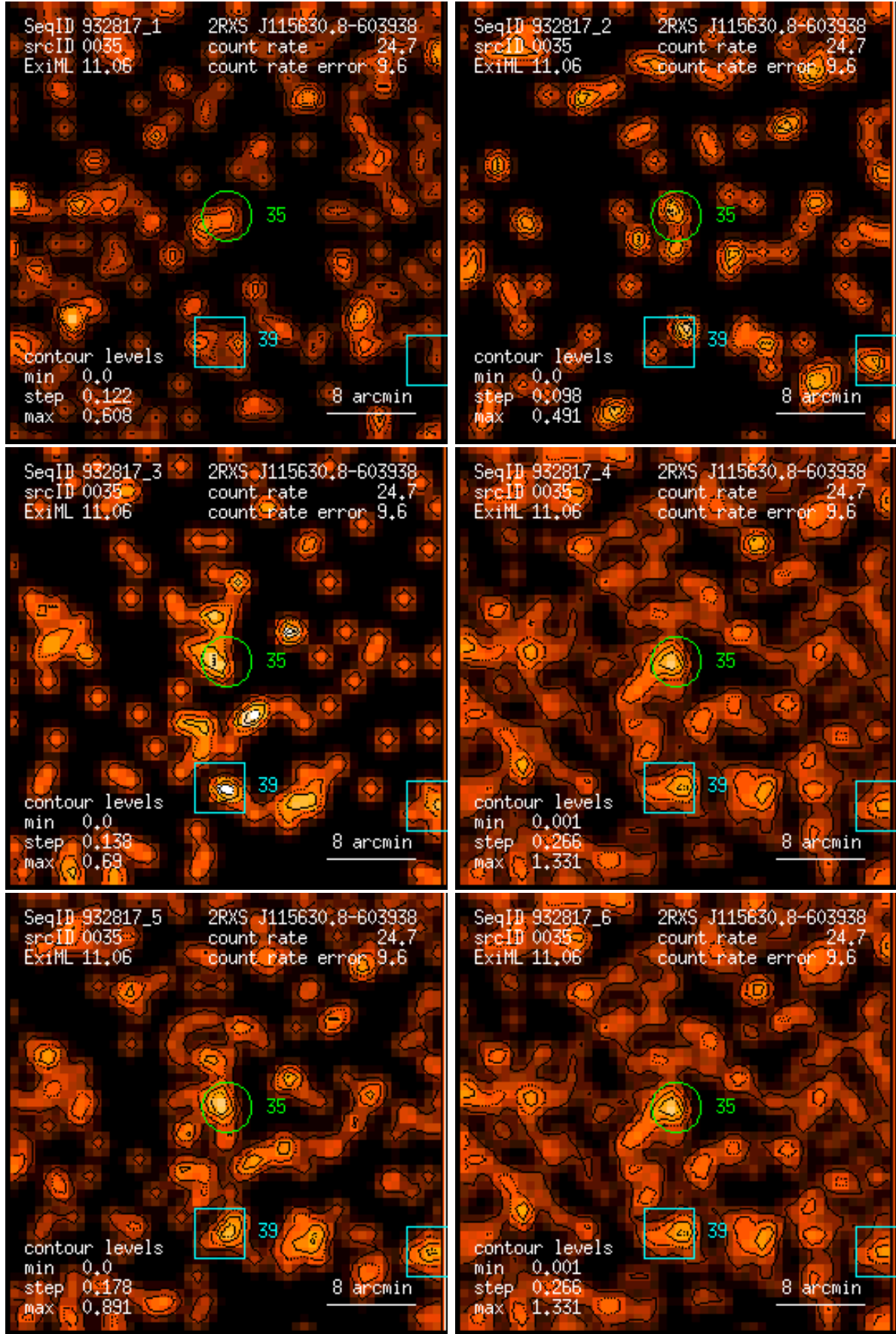
Figure 35: RASS 932817: detection 0035: band rate images, Gaussian filter: (1) PSPC channels 11 – 41, (2) 52 – 90, (3) 91 – 201, (4) 11 – 235, (5) 52 – 201, (6) 11 – 201. Broad band rates in counts/ks. Band rate contour levels in counts/ks/arcmin 2 .
