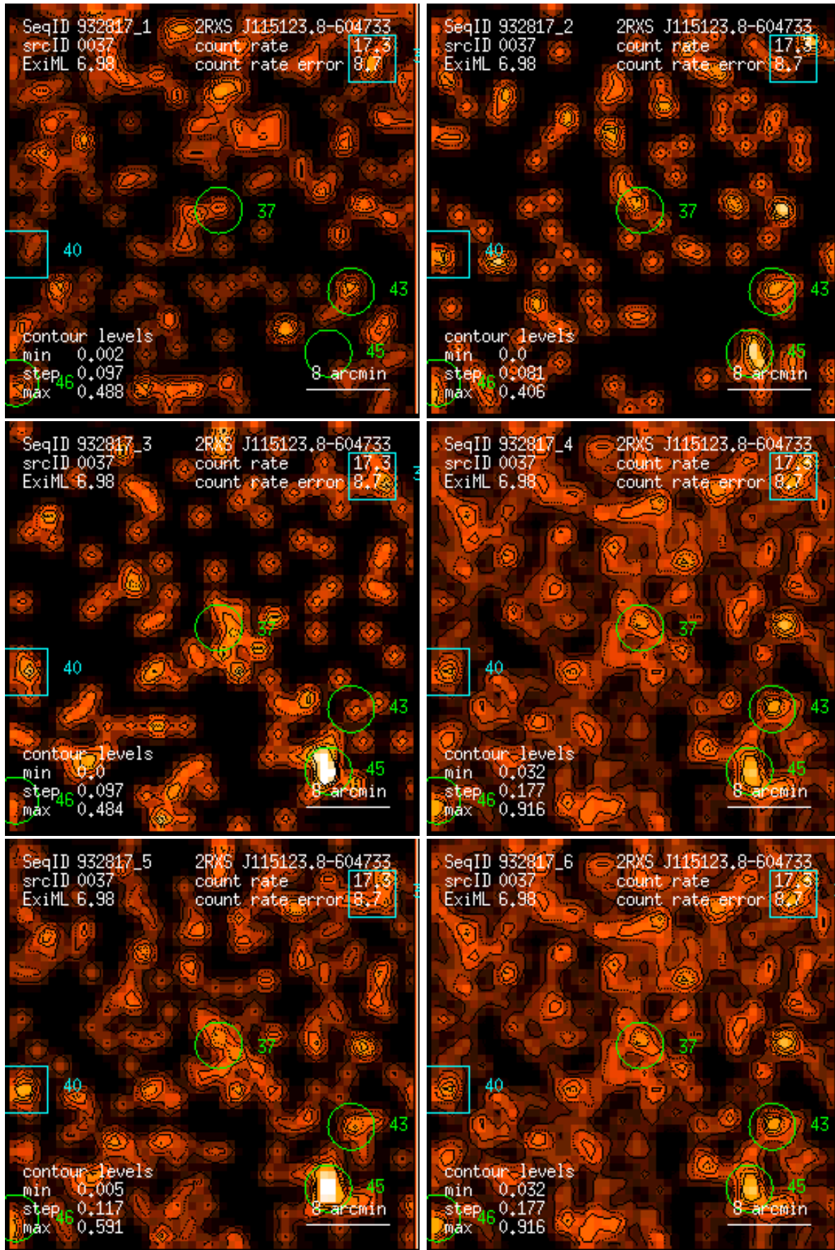
Figure 37: RASS 932817: detection 0037: band rate images, Gaussian filter: (1) PSPC channels 11 – 41, (2) 52 – 90, (3) 91 – 201, (4) 11 – 235, (5) 52 – 201, (6) 11 – 201. Broad band rates in counts/ks. Band rate contour levels in counts/ks/arcmin 2 .
