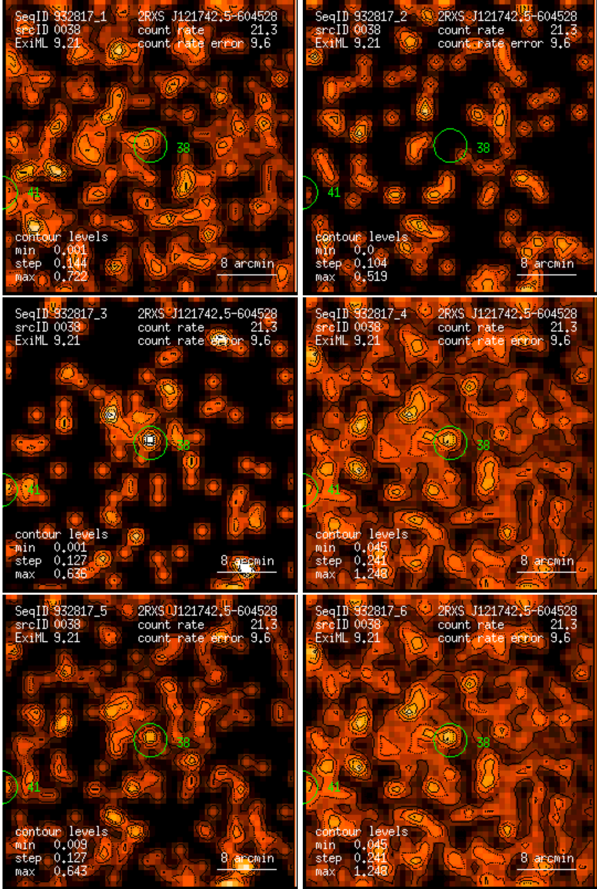
Figure 38: RASS 932817: detection 0038: band rate images, Gaussian filter: (1) PSPC channels 11 – 41, (2) 52 – 90, (3) 91 – 201, (4) 11 – 235, (5) 52 – 201, (6) 11 – 201. Broad band rates in counts/ks. Band rate contour levels in counts/ks/arcmin 2 .
