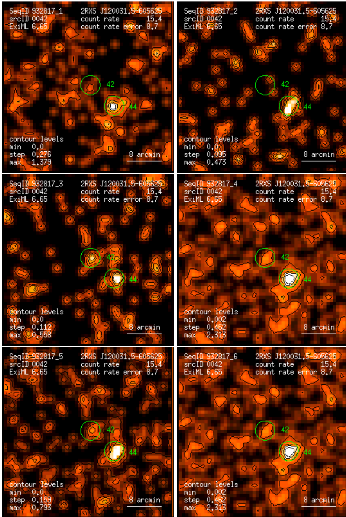
Figure 42: RASS 932817: detection 0042: band rate images, Gaussian filter: (1) PSPC channels 11 – 41, (2) 52 – 90, (3) 91 – 201, (4) 11 – 235, (5) 52 – 201, (6) 11 – 201. Broad band rates in counts/ks. Band rate contour levels in counts/ks/arcmin 2 .
