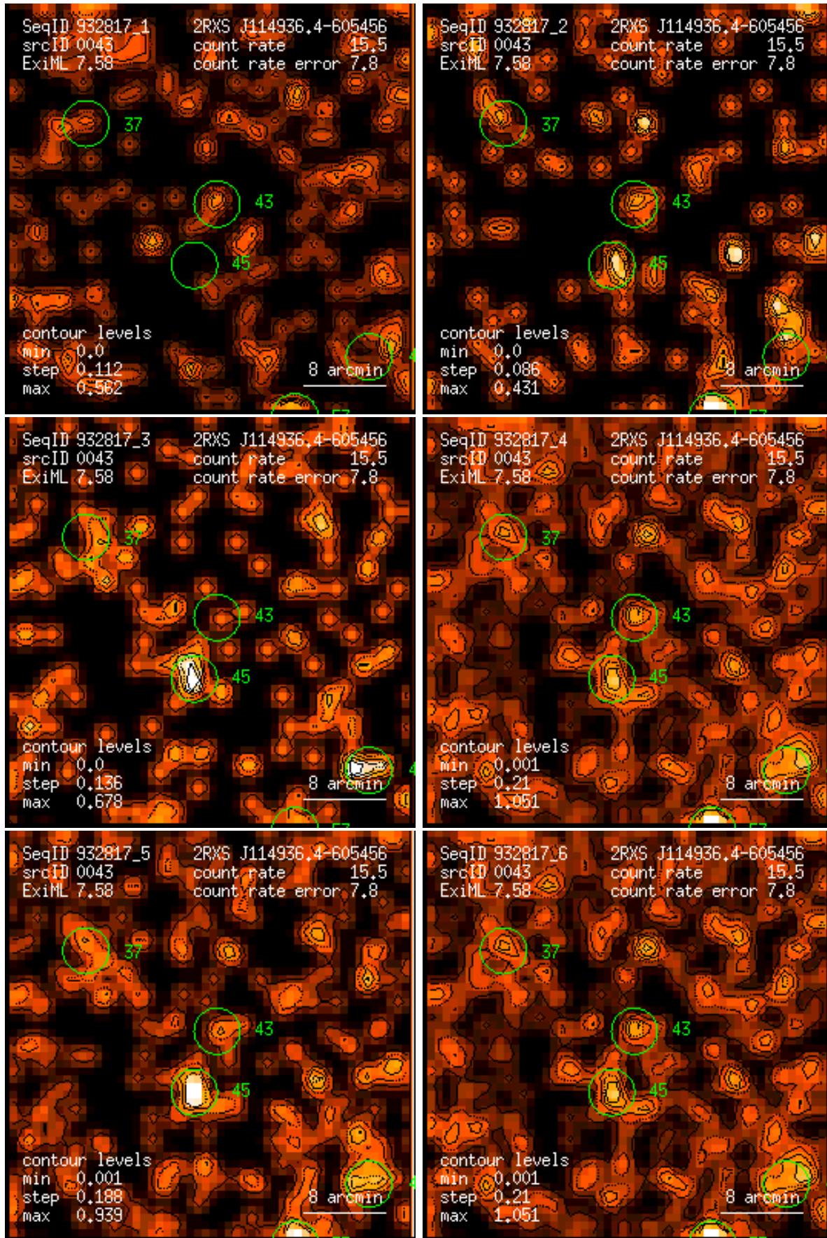
Figure 43: RASS 932817: detection 0043: band rate images, Gaussian filter: (1) PSPC channels 11 – 41, (2) 52 – 90, (3) 91 – 201, (4) 11 – 235, (5) 52 – 201, (6) 11 – 201. Broad band rates in counts/ks. Band rate contour levels in counts/ks/arcmin 2 .
