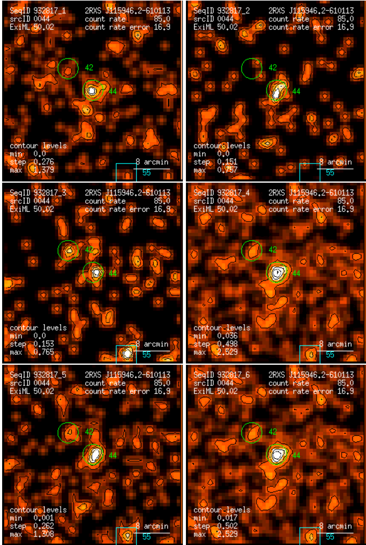
Figure 44: RASS 932817: detection 0044: band rate images, Gaussian filter: (1) PSPC channels 11 – 41, (2) 52 – 90, (3) 91 – 201, (4) 11 – 235, (5) 52 – 201, (6) 11 – 201. Broad band rates in counts/ks. Band rate contour levels in counts/ks/arcmin 2 .
