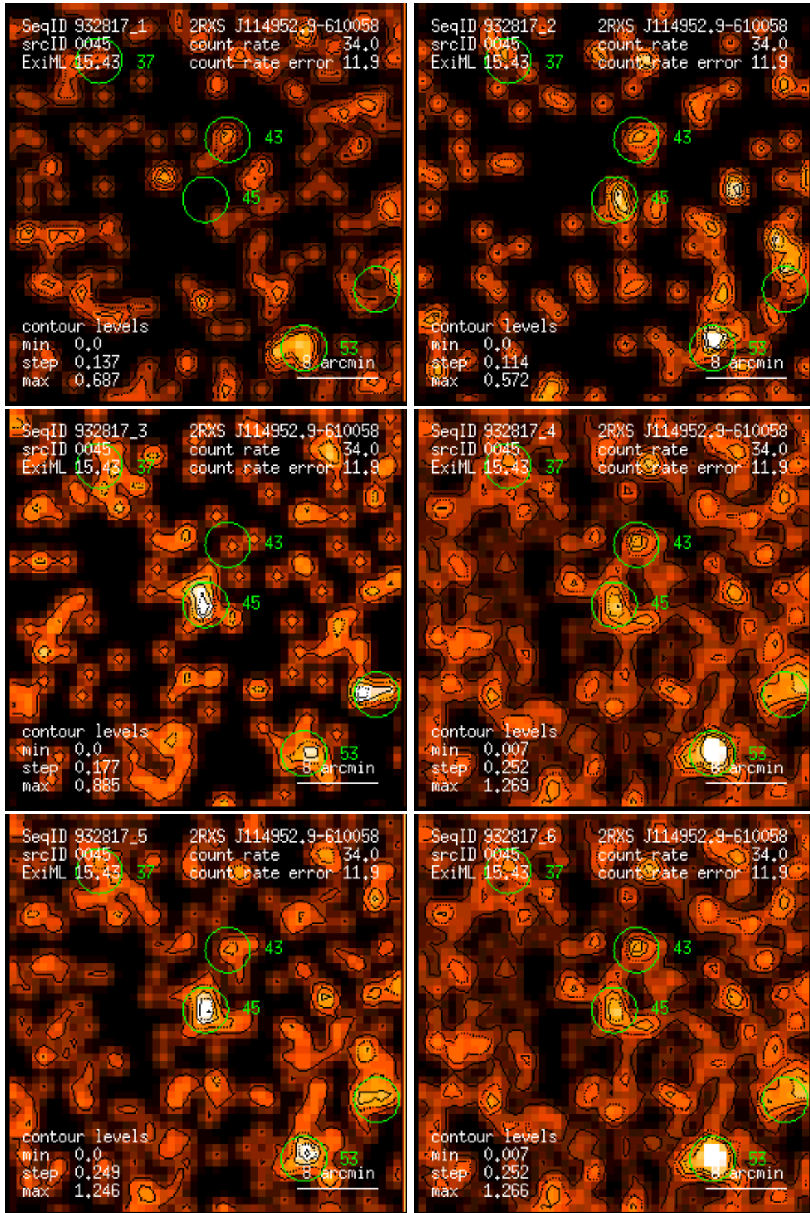
Figure 45: RASS 932817: detection 0045: band rate images, Gaussian filter: (1) PSPC channels 11 – 41, (2) 52 – 90, (3) 91 – 201, (4) 11 – 235, (5) 52 – 201, (6) 11 – 201. Broad band rates in counts/ks. Band rate contour levels in counts/ks/arcmin 2 .
