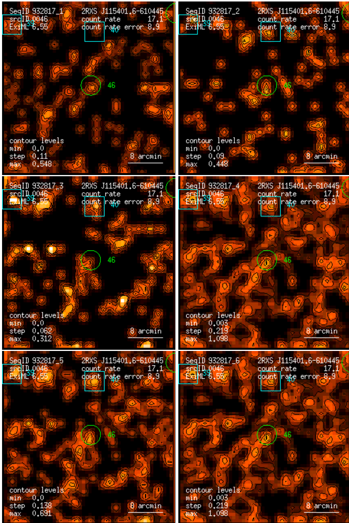
Figure 46: RASS 932817: detection 0046: band rate images, Gaussian filter: (1) PSPC channels 11 – 41, (2) 52 – 90, (3) 91 – 201, (4) 11 – 235, (5) 52 – 201, (6) 11 – 201. Broad band rates in counts/ks. Band rate contour levels in counts/ks/arcmin 2 .
