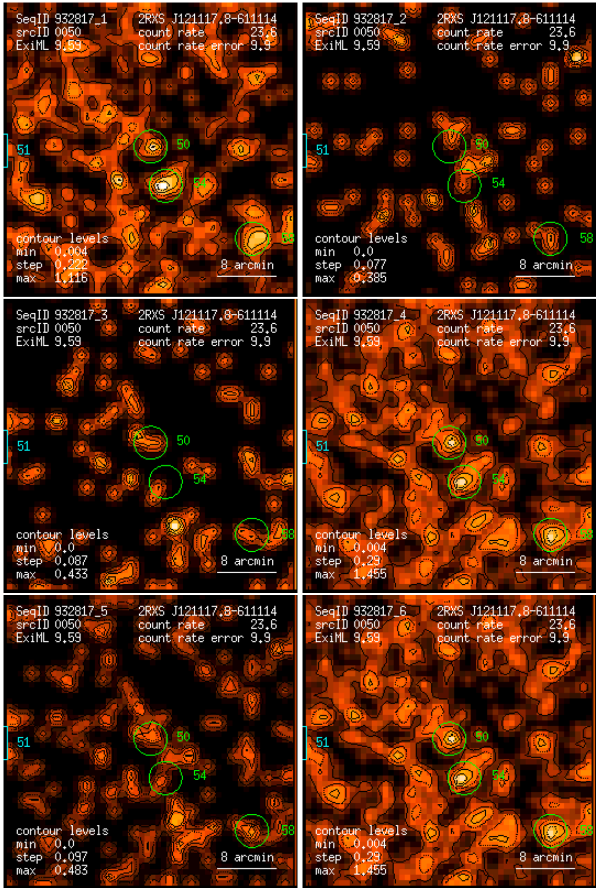
Figure 50: RASS 932817: detection 0050: band rate images, Gaussian filter: (1) PSPC channels 11 – 41, (2) 52 – 90, (3) 91 – 201, (4) 11 – 235, (5) 52 – 201, (6) 11 – 201. Broad band rates in counts/ks. Band rate contour levels in counts/ks/arcmin 2 .
