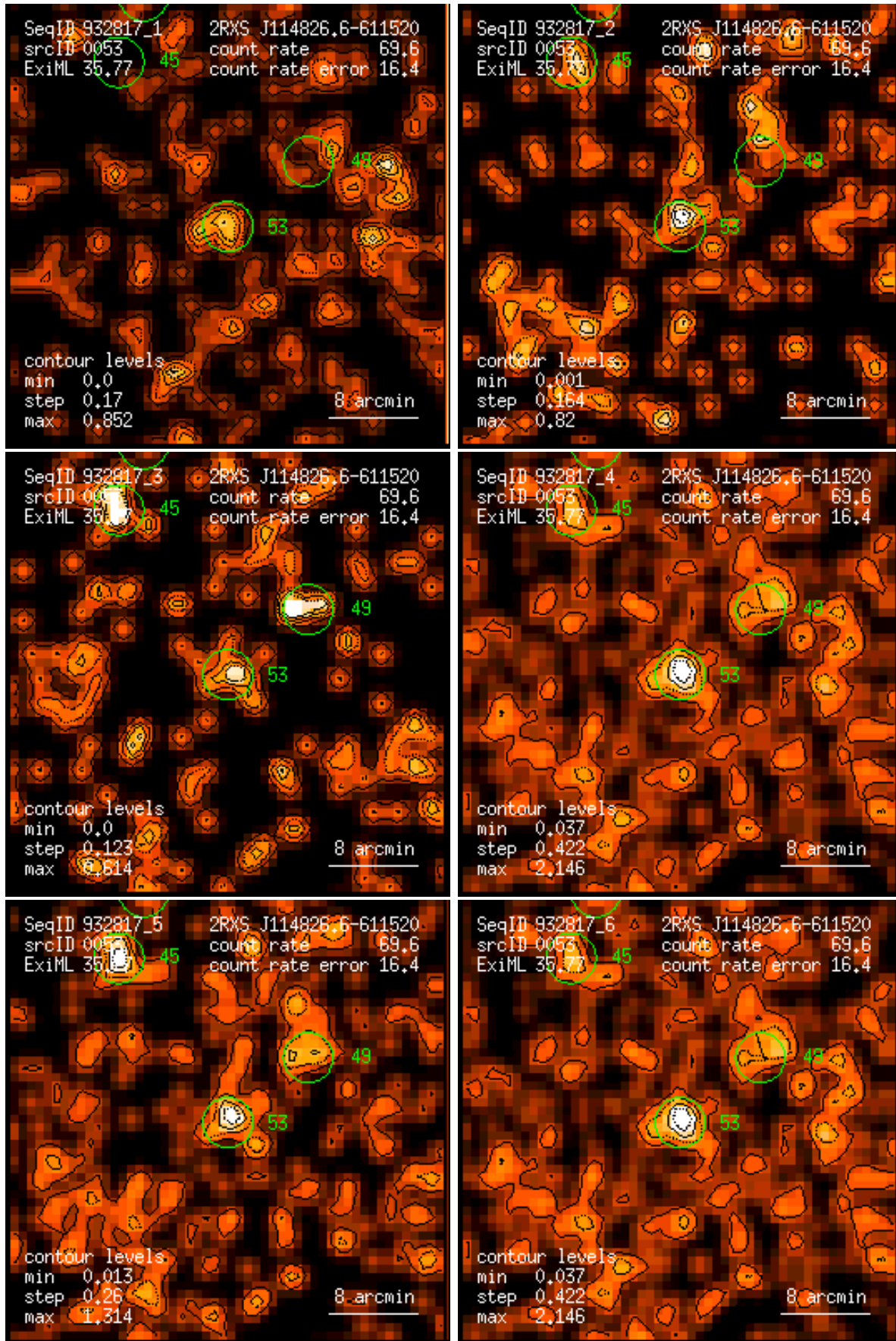
Figure 53: RASS 932817: detection 0053: band rate images, Gaussian filter: (1) PSPC channels 11 – 41, (2) 52 – 90, (3) 91 – 201, (4) 11 – 235, (5) 52 – 201, (6) 11 – 201. Broad band rates in counts/ks. Band rate contour levels in counts/ks/arcmin 2 .
