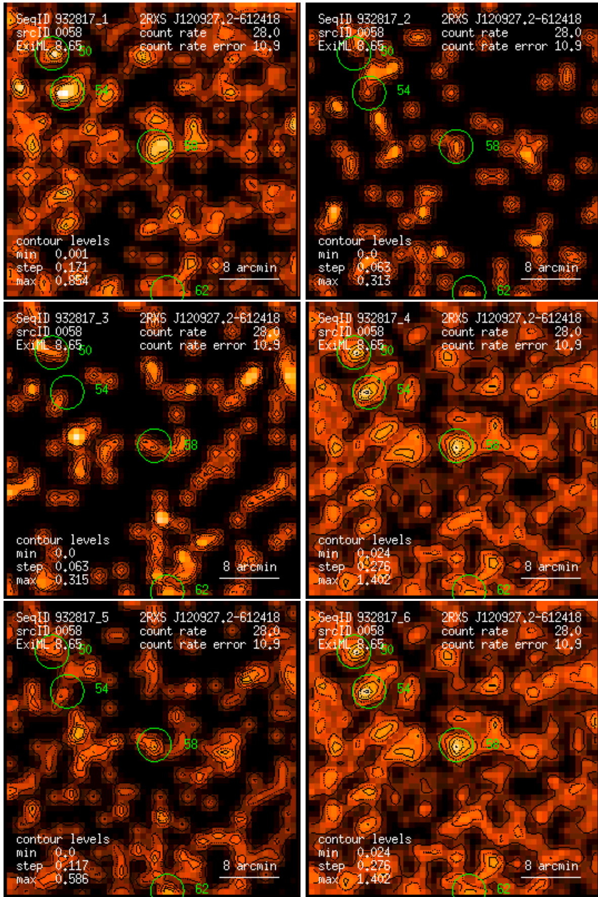
Figure 58: RASS 932817: detection 0058: band rate images, Gaussian filter: (1) PSPC channels 11 – 41, (2) 52 – 90, (3) 91 – 201, (4) 11 – 235, (5) 52 – 201, (6) 11 – 201. Broad band rates in counts/ks. Band rate contour levels in counts/ks/arcmin 2 .
