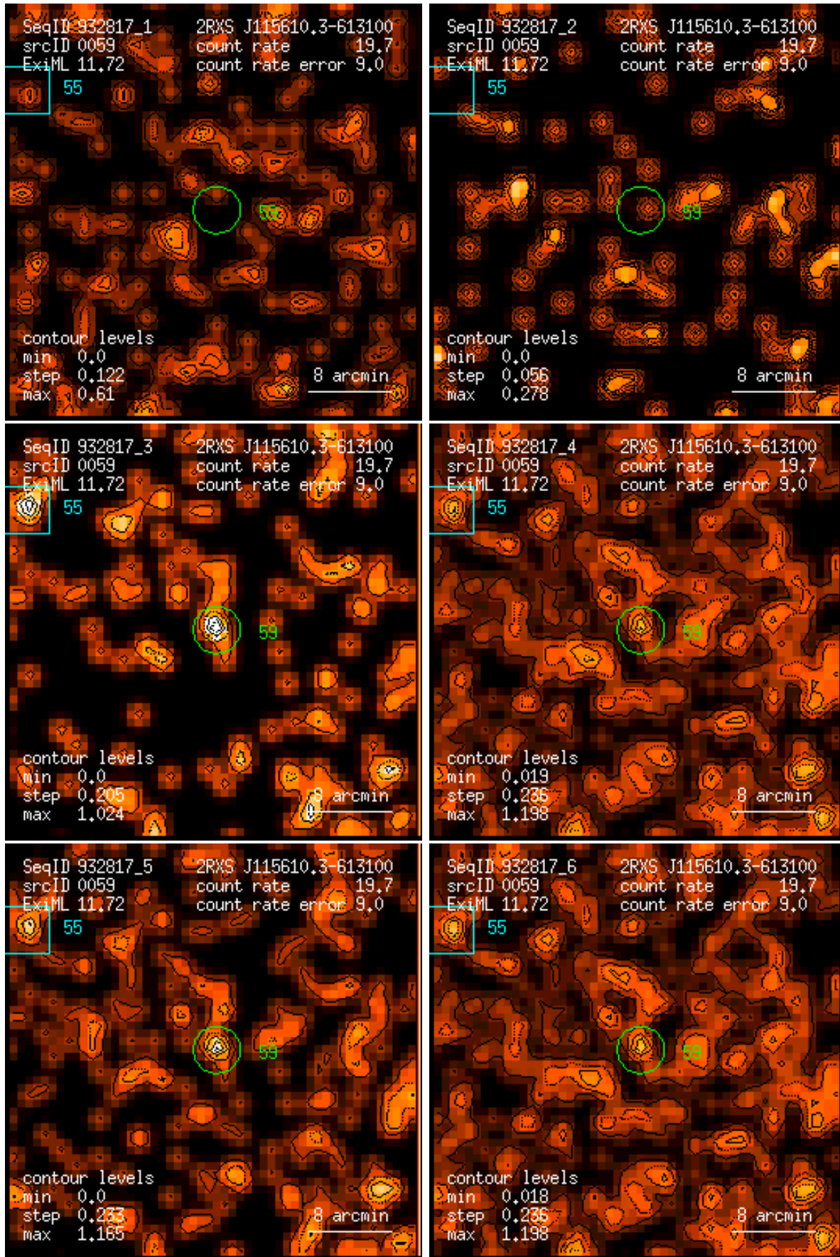
Figure 59: RASS 932817: detection 0059: band rate images, Gaussian filter: (1) PSPC channels 11 – 41, (2) 52 – 90, (3) 91 – 201, (4) 11 – 235, (5) 52 – 201, (6) 11 – 201. Broad band rates in counts/ks. Band rate contour levels in counts/ks/arcmin 2 .
