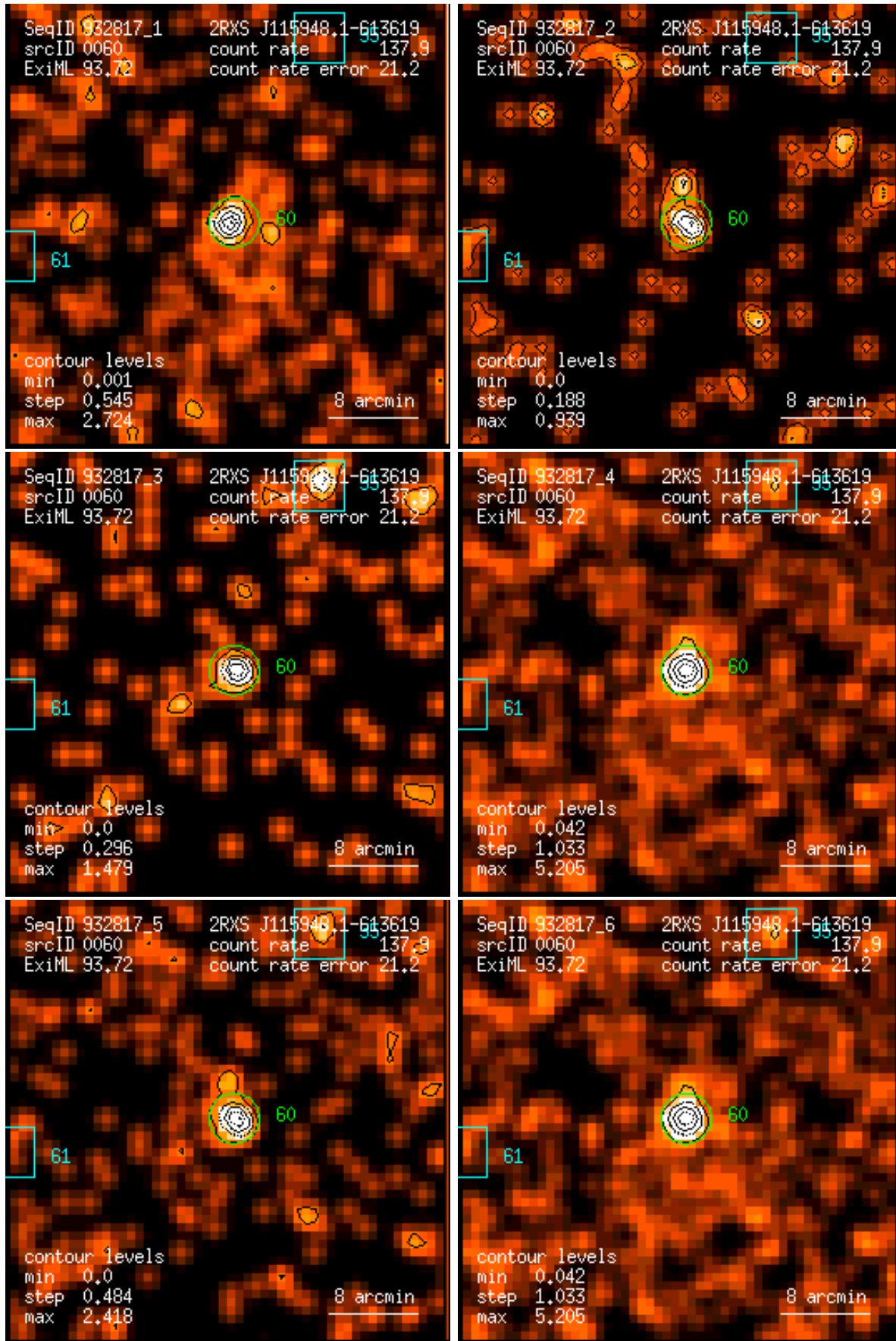
Figure 60: RASS 932817: detection 0060: band rate images, Gaussian filter: (1) PSPC channels 11 – 41, (2) 52 – 90, (3) 91 – 201, (4) 11 – 235, (5) 52 – 201, (6) 11 – 201. Broad band rates in counts/ks. Band rate contour levels in counts/ks/arcmin 2 .
