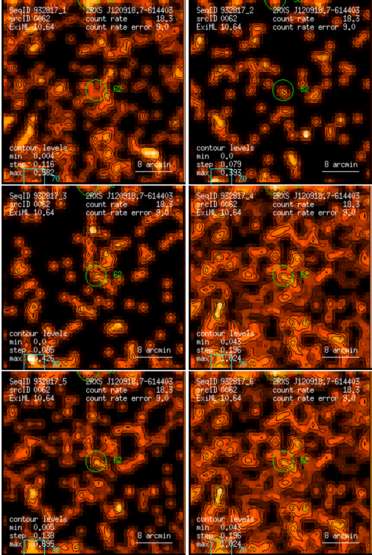
Figure 62: RASS 932817: detection 0062: band rate images, Gaussian filter: (1) PSPC channels 11 – 41, (2) 52 – 90, (3) 91 – 201, (4) 11 – 235, (5) 52 – 201, (6) 11 – 201. Broad band rates in counts/ks. Band rate contour levels in counts/ks/arcmin 2 .
