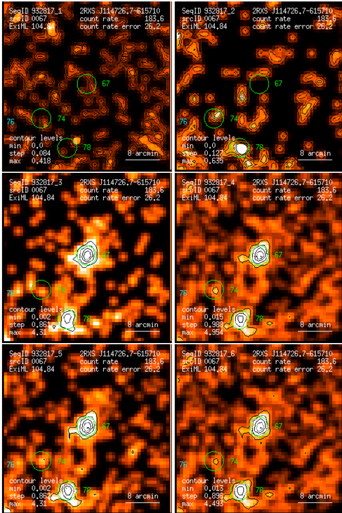
Figure 67: RASS 932817: detection 0067: band rate images, Gaussian filter: (1) PSPC channels 11 – 41, (2) 52 – 90, (3) 91 – 201, (4) 11 – 235, (5) 52 – 201, (6) 11 – 201. Broad band rates in counts/ks. Band rate contour levels in counts/ks/arcmin 2 .
