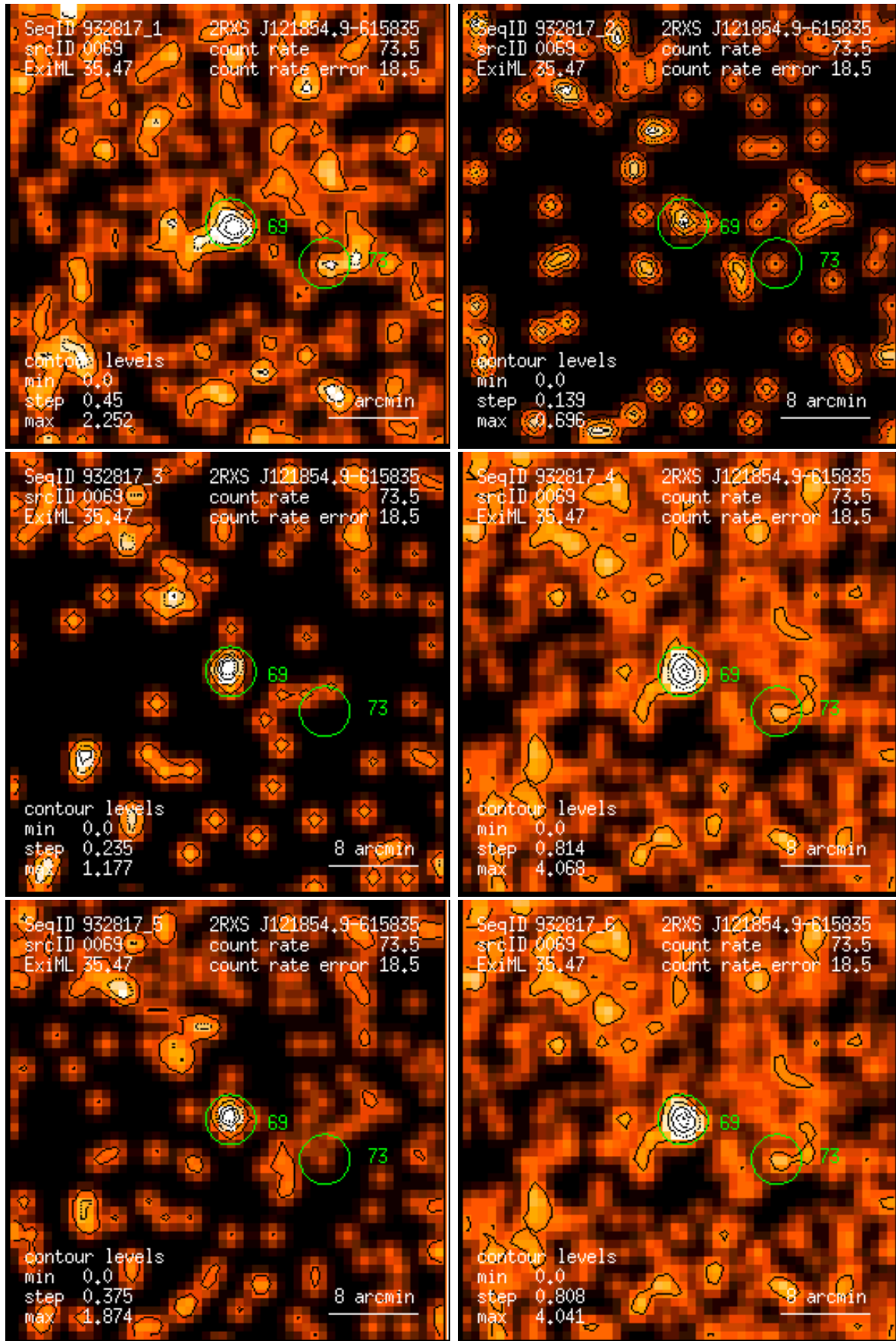
Figure 69: RASS 932817: detection 0069: band rate images, Gaussian filter: (1) PSPC channels 11 – 41, (2) 52 – 90, (3) 91 – 201, (4) 11 – 235, (5) 52 – 201, (6) 11 – 201. Broad band rates in counts/ks. Band rate contour levels in counts/ks/arcmin 2 .
