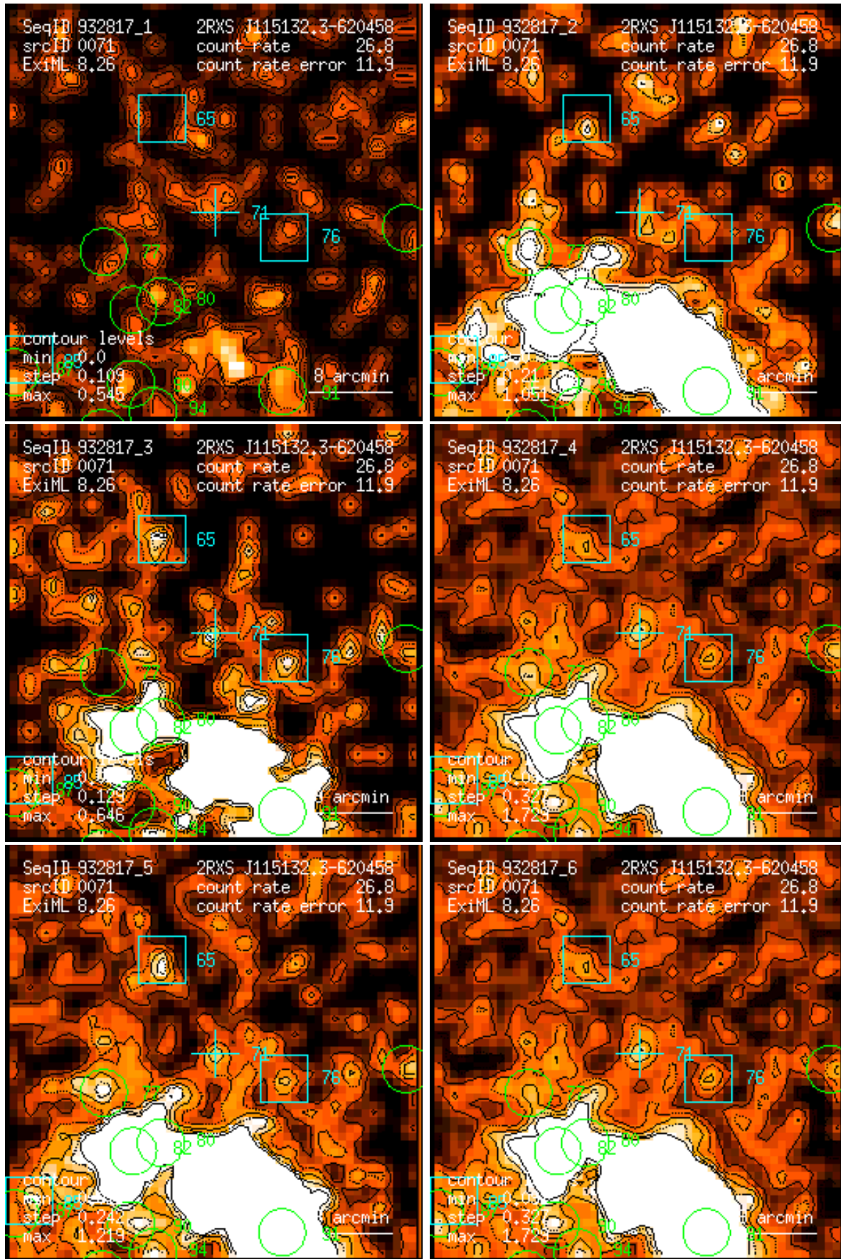
Figure 71: RASS 932817: detection 0071: band rate images, Gaussian filter: (1) PSPC channels 11 – 41, (2) 52 – 90, (3) 91 – 201, (4) 11 – 235, (5) 52 – 201, (6) 11 – 201. Broad band rates in counts/ks. Band rate contour levels in counts/ks/arcmin 2 .
