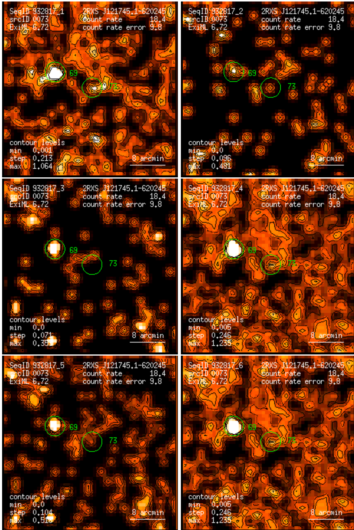
Figure 73: RASS 932817: detection 0073: band rate images, Gaussian filter: (1) PSPC channels 11 – 41, (2) 52 – 90, (3) 91 – 201, (4) 11 – 235, (5) 52 – 201, (6) 11 – 201. Broad band rates in counts/ks. Band rate contour levels in counts/ks/arcmin 2 .
