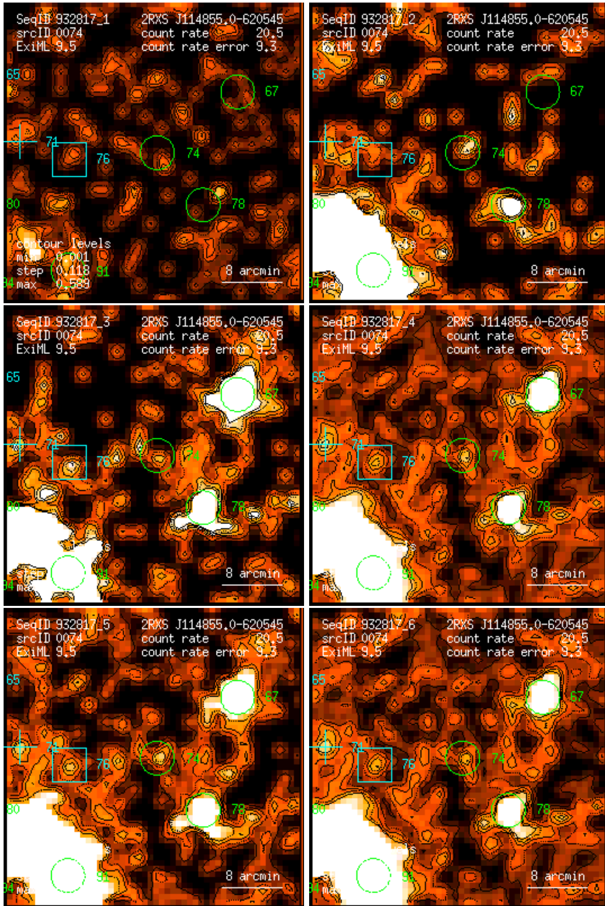
Figure 74: RASS 932817: detection 0074: band rate images, Gaussian filter: (1) PSPC channels 11 – 41, (2) 52 – 90, (3) 91 – 201, (4) 11 – 235, (5) 52 – 201, (6) 11 – 201. Broad band rates in counts/ks. Band rate contour levels in counts/ks/arcmin 2 .
