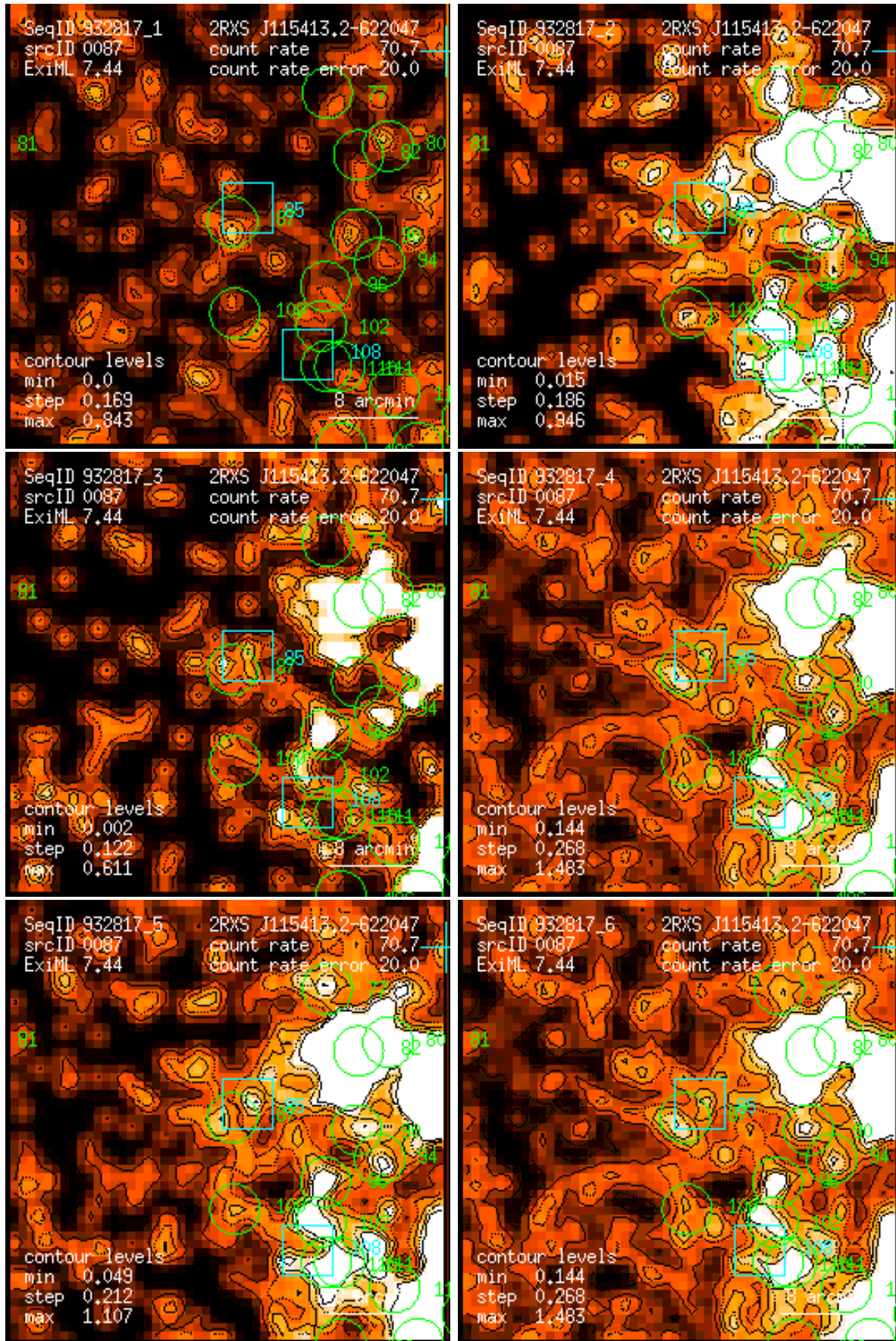
Figure 87: RASS 932817: detection 0087: band rate images, Gaussian filter: (1) PSPC channels 11 – 41, (2) 52 – 90, (3) 91 – 201, (4) 11 – 235, (5) 52 – 201, (6) 11 – 201. Broad band rates in counts/ks. Band rate contour levels in counts/ks/arcmin 2 .
