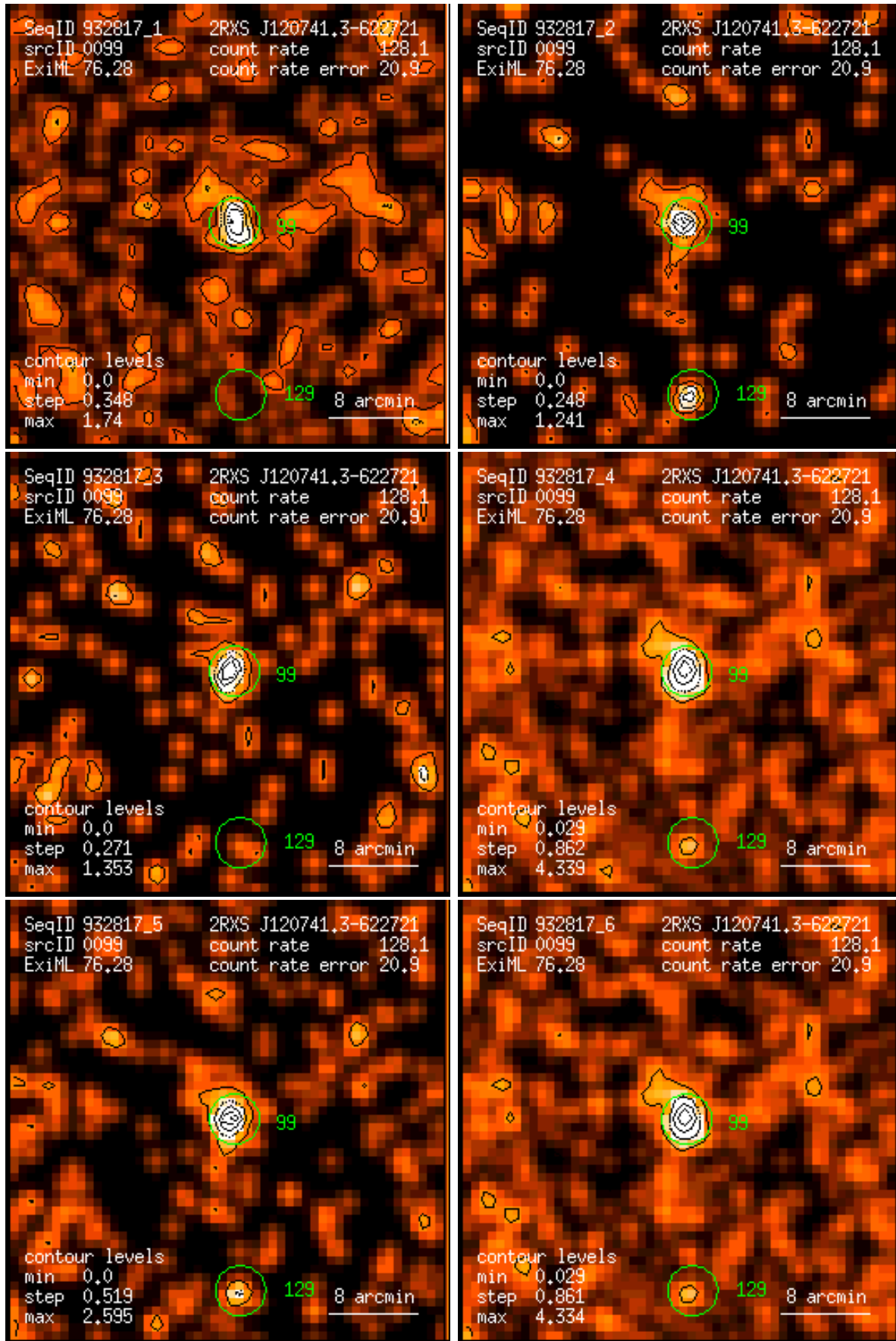
Figure 99: RASS 932817: detection 0099: band rate images, Gaussian filter: (1) PSPC channels 11 – 41, (2) 52 – 90, (3) 91 – 201, (4) 11 – 235, (5) 52 – 201, (6) 11 – 201. Broad band rates in counts/ks. Band rate contour levels in counts/ks/arcmin 2 .
