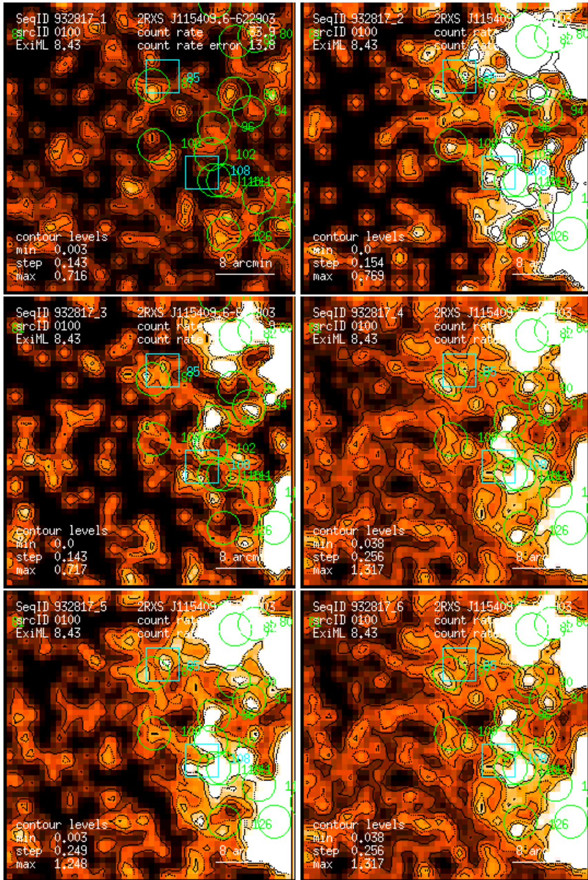
Figure 100: RASS 932817: detection 0100: band rate images, Gaussian filter: (1) PSPC channels 11 – 41, (2) 52 – 90, (3) 91 – 201, (4) 11 – 235, (5) 52 – 201, (6) 11 – 201. Broad band rates in counts/ks. Band rate contour levels in counts/ks/arcmin 2 .
