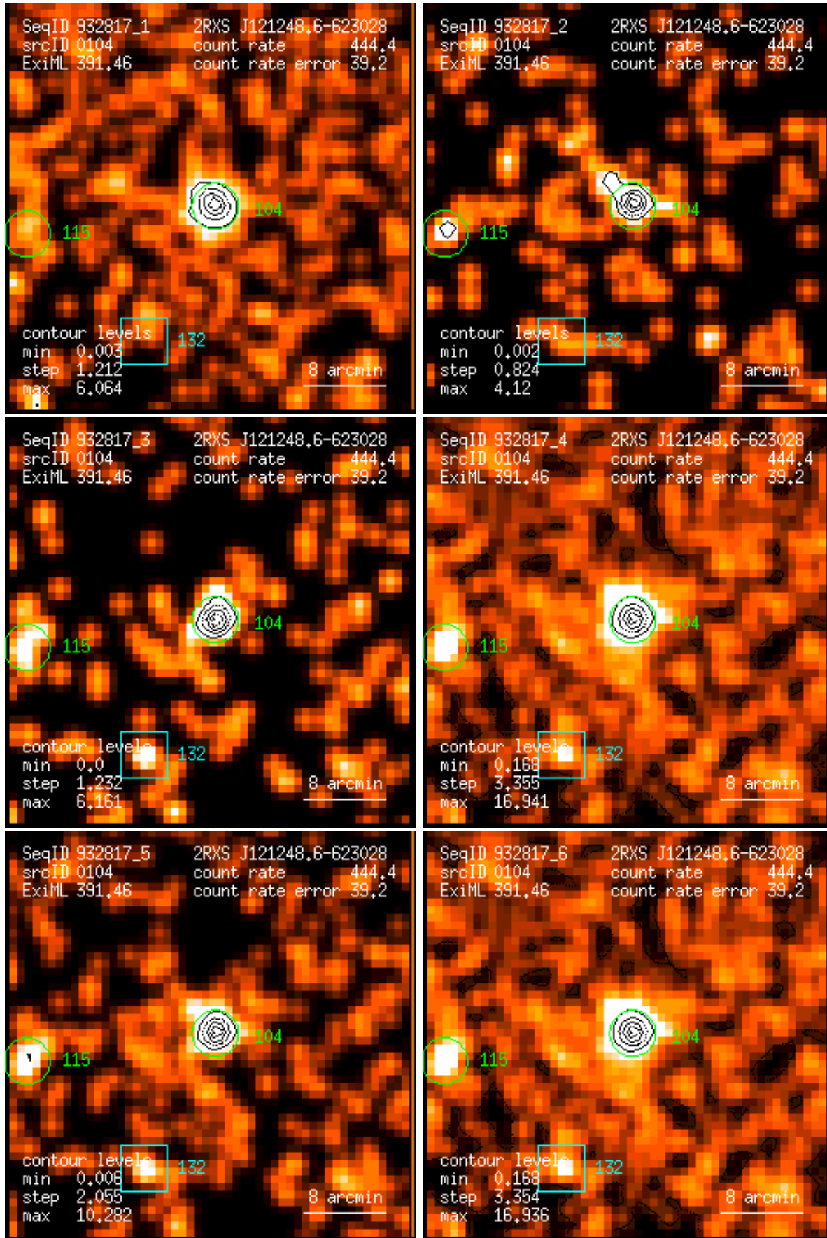
Figure 104: RASS 932817: detection 0104: band rate images, Gaussian filter: (1) PSPC channels 11 – 41, (2) 52 – 90, (3) 91 – 201, (4) 11 – 235, (5) 52 – 201, (6) 11 – 201. Broad band rates in counts/ks. Band rate contour levels in counts/ks/arcmin 2 .
