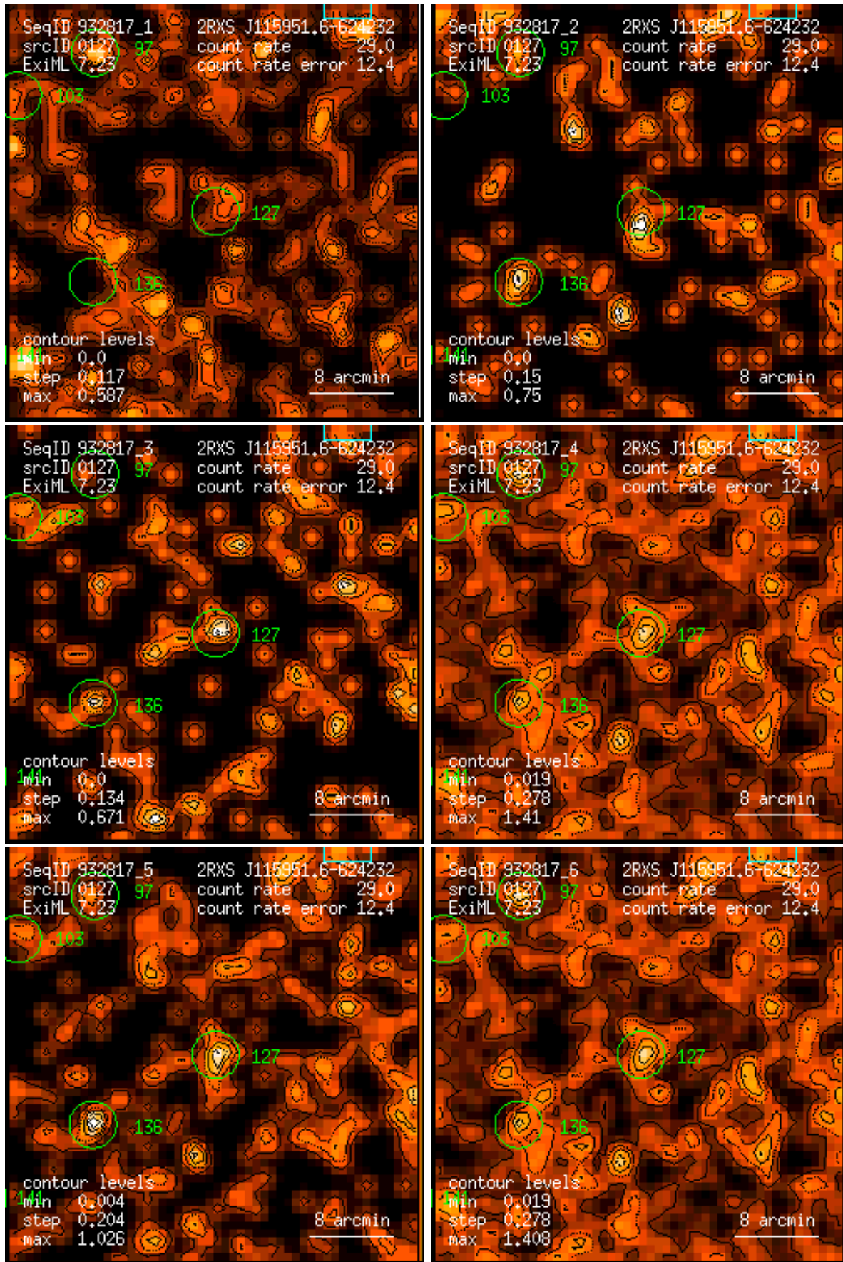
Figure 127: RASS 932817: detection 0127: band rate images, Gaussian filter: (1) PSPC channels 11 – 41, (2) 52 – 90, (3) 91 – 201, (4) 11 – 235, (5) 52 – 201, (6) 11 – 201. Broad band rates in counts/ks. Band rate contour levels in counts/ks/arcmin 2 .
