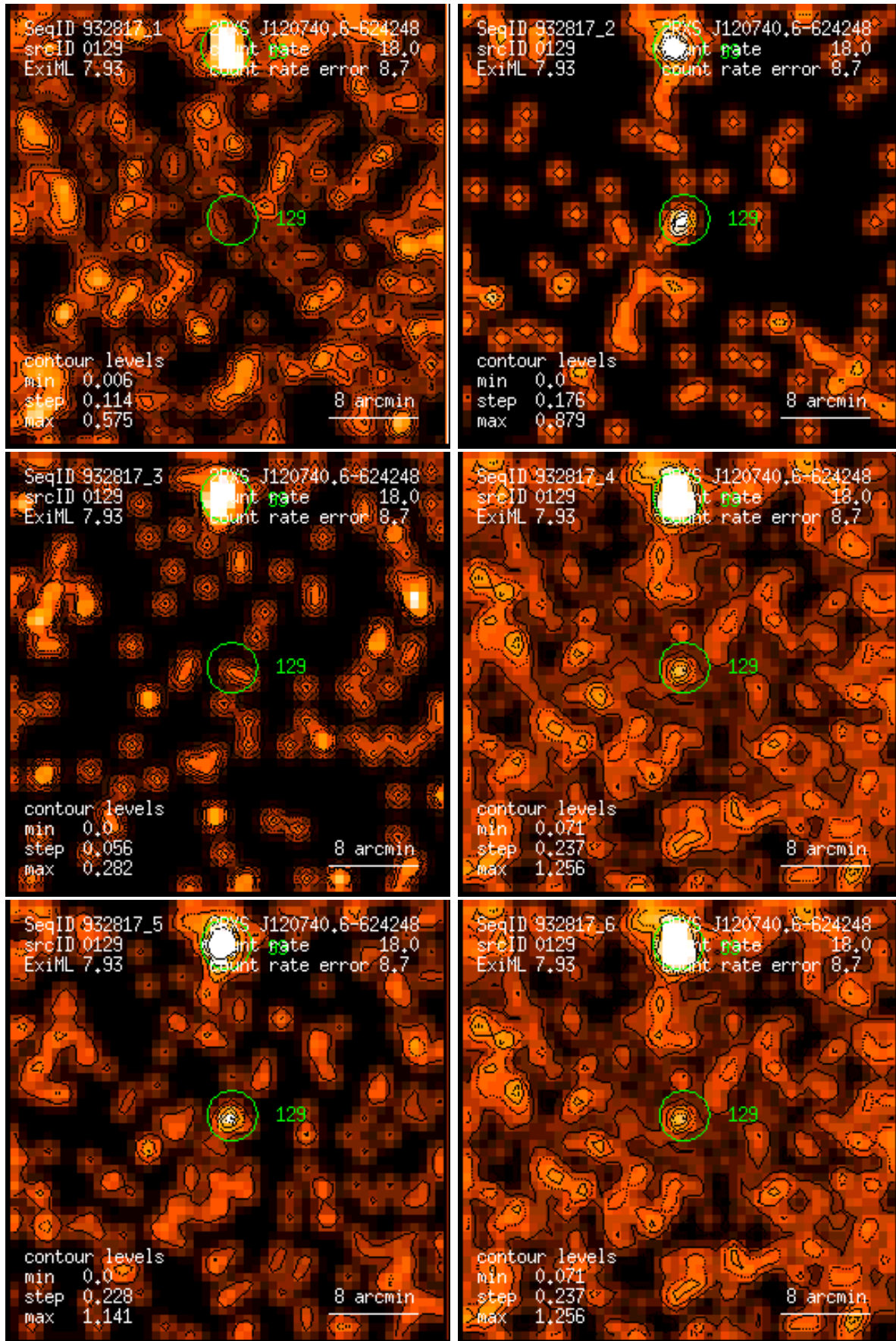
Figure 129: RASS 932817: detection 0129: band rate images, Gaussian filter: (1) PSPC channels 11 – 41, (2) 52 – 90, (3) 91 – 201, (4) 11 – 235, (5) 52 – 201, (6) 11 – 201. Broad band rates in counts/ks. Band rate contour levels in counts/ks/arcmin 2 .
