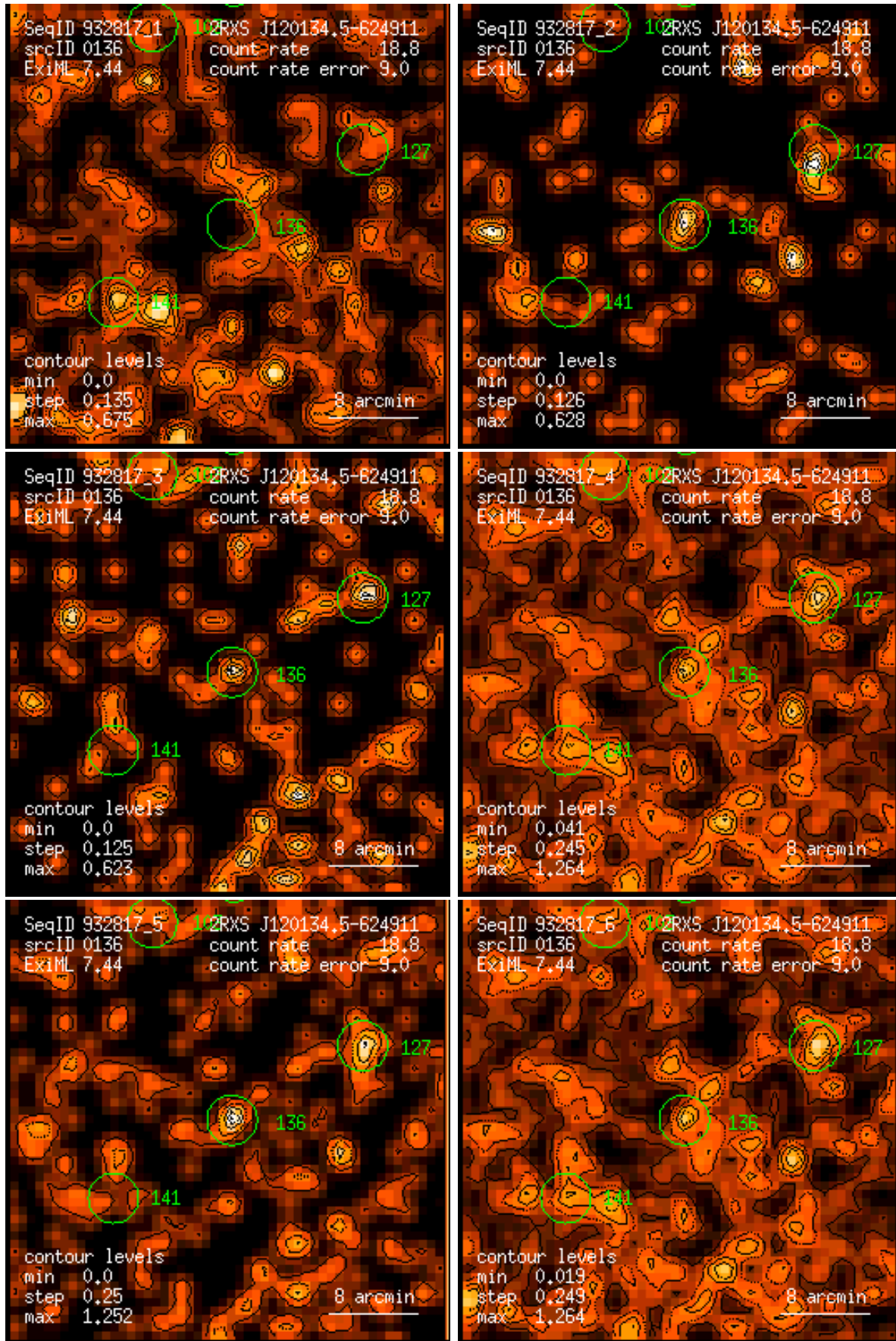
Figure 136: RASS 932817: detection 0136: band rate images, Gaussian filter: (1) PSPC channels 11 – 41, (2) 52 – 90, (3) 91 – 201, (4) 11 – 235, (5) 52 – 201, (6) 11 – 201. Broad band rates in counts/ks. Band rate contour levels in counts/ks/arcmin 2 .
