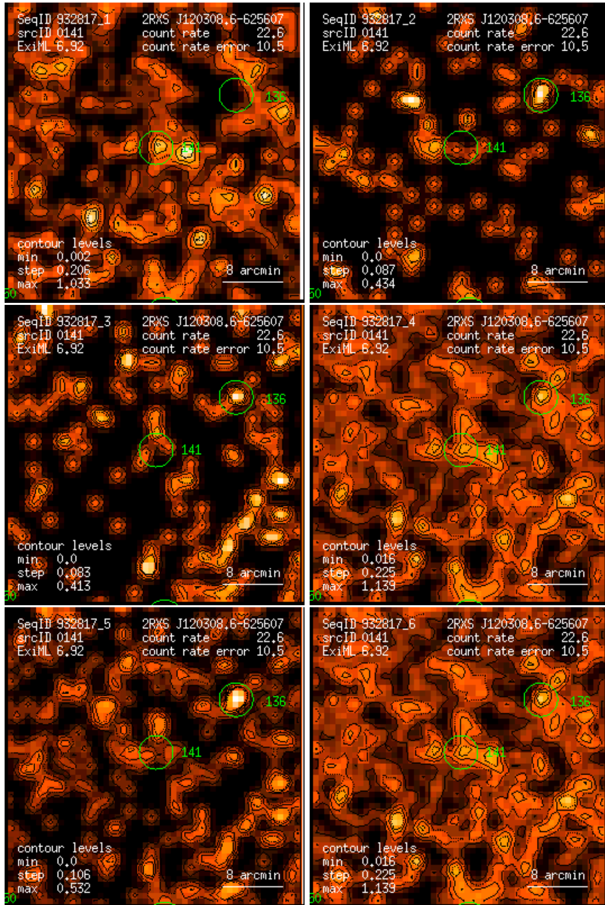
Figure 141: RASS 932817: detection 0141: band rate images, Gaussian filter: (1) PSPC channels 11 – 41, (2) 52 – 90, (3) 91 – 201, (4) 11 – 235, (5) 52 – 201, (6) 11 – 201. Broad band rates in counts/ks. Band rate contour levels in counts/ks/arcmin 2 .
