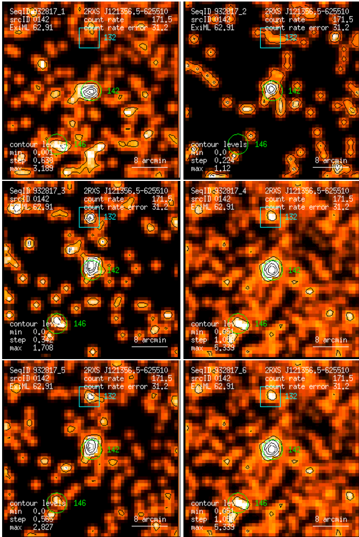
Figure 142: RASS 932817: detection 0142: band rate images, Gaussian filter: (1) PSPC channels 11 – 41, (2) 52 – 90, (3) 91 – 201, (4) 11 – 235, (5) 52 – 201, (6) 11 – 201. Broad band rates in counts/ks. Band rate contour levels in counts/ks/arcmin 2 .
