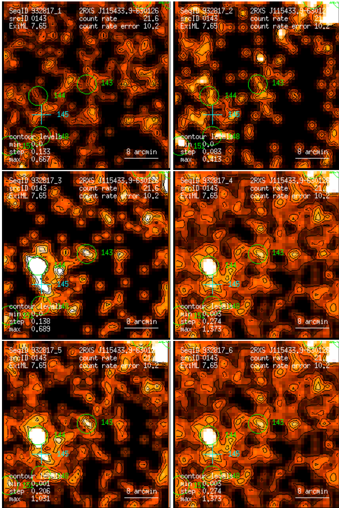
Figure 143: RASS 932817: detection 0143: band rate images, Gaussian filter: (1) PSPC channels 11 – 41, (2) 52 – 90, (3) 91 – 201, (4) 11 – 235, (5) 52 – 201, (6) 11 – 201. Broad band rates in counts/ks. Band rate contour levels in counts/ks/arcmin 2 .
