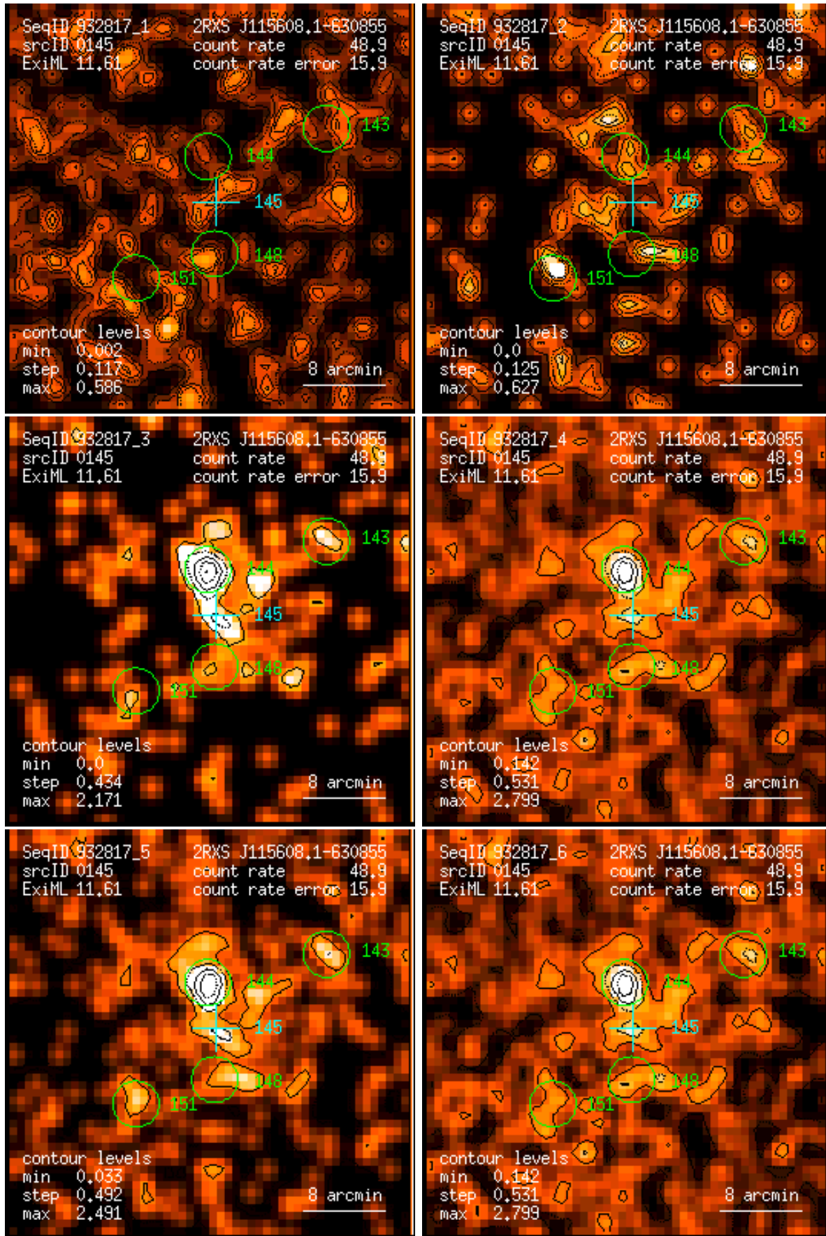
Figure 145: RASS 932817: detection 0145: band rate images, Gaussian filter: (1) PSPC channels 11 – 41, (2) 52 – 90, (3) 91 – 201, (4) 11 – 235, (5) 52 – 201, (6) 11 – 201. Broad band rates in counts/ks. Band rate contour levels in counts/ks/arcmin 2 .
