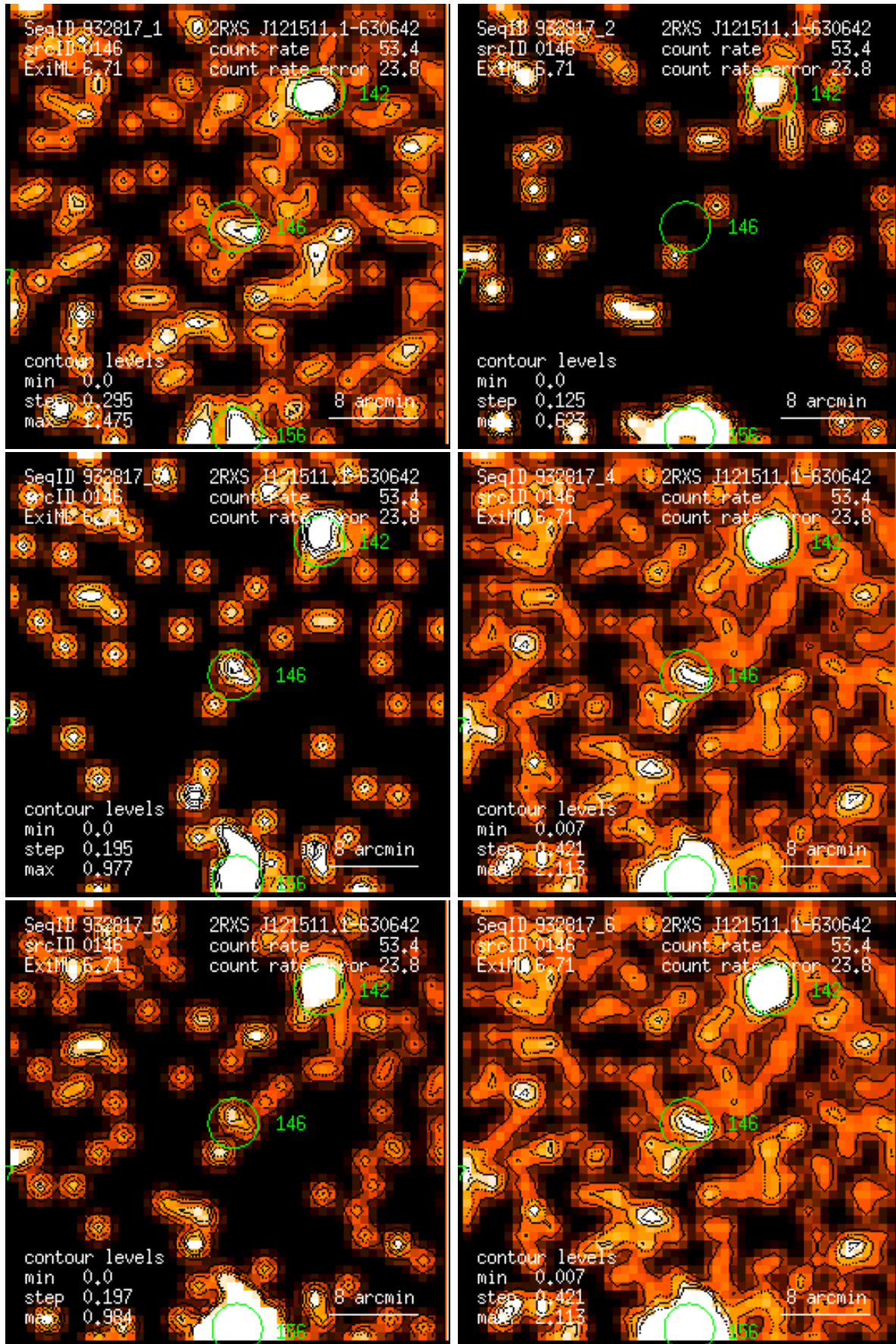
Figure 146: RASS 932817: detection 0146: band rate images, Gaussian filter: (1) PSPC channels 11 – 41, (2) 52 – 90, (3) 91 – 201, (4) 11 – 235, (5) 52 – 201, (6) 11 – 201. Broad band rates in counts/ks. Band rate contour levels in counts/ks/arcmin 2 .
