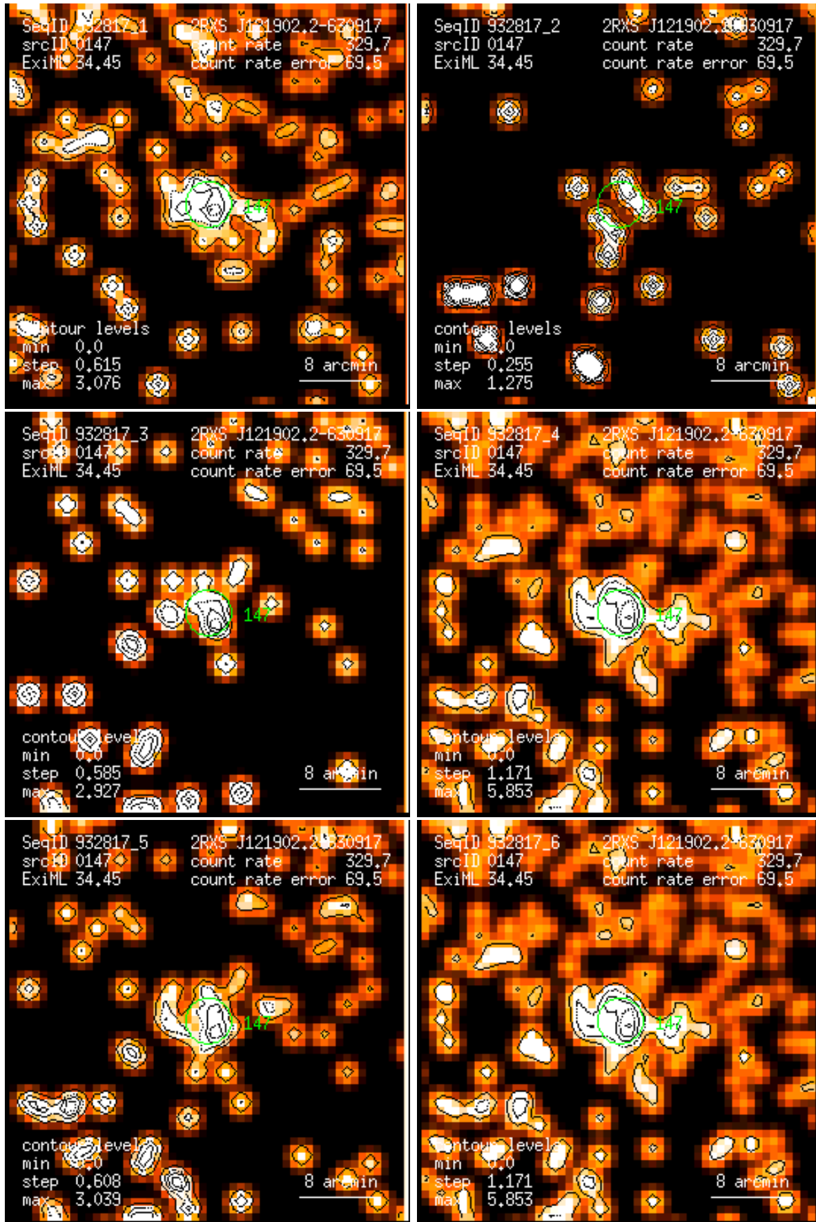
Figure 147: RASS 932817: detection 0147: band rate images, Gaussian filter: (1) PSPC channels 11 – 41, (2) 52 – 90, (3) 91 – 201, (4) 11 – 235, (5) 52 – 201, (6) 11 – 201. Broad band rates in counts/ks. Band rate contour levels in counts/ks/arcmin 2 .
