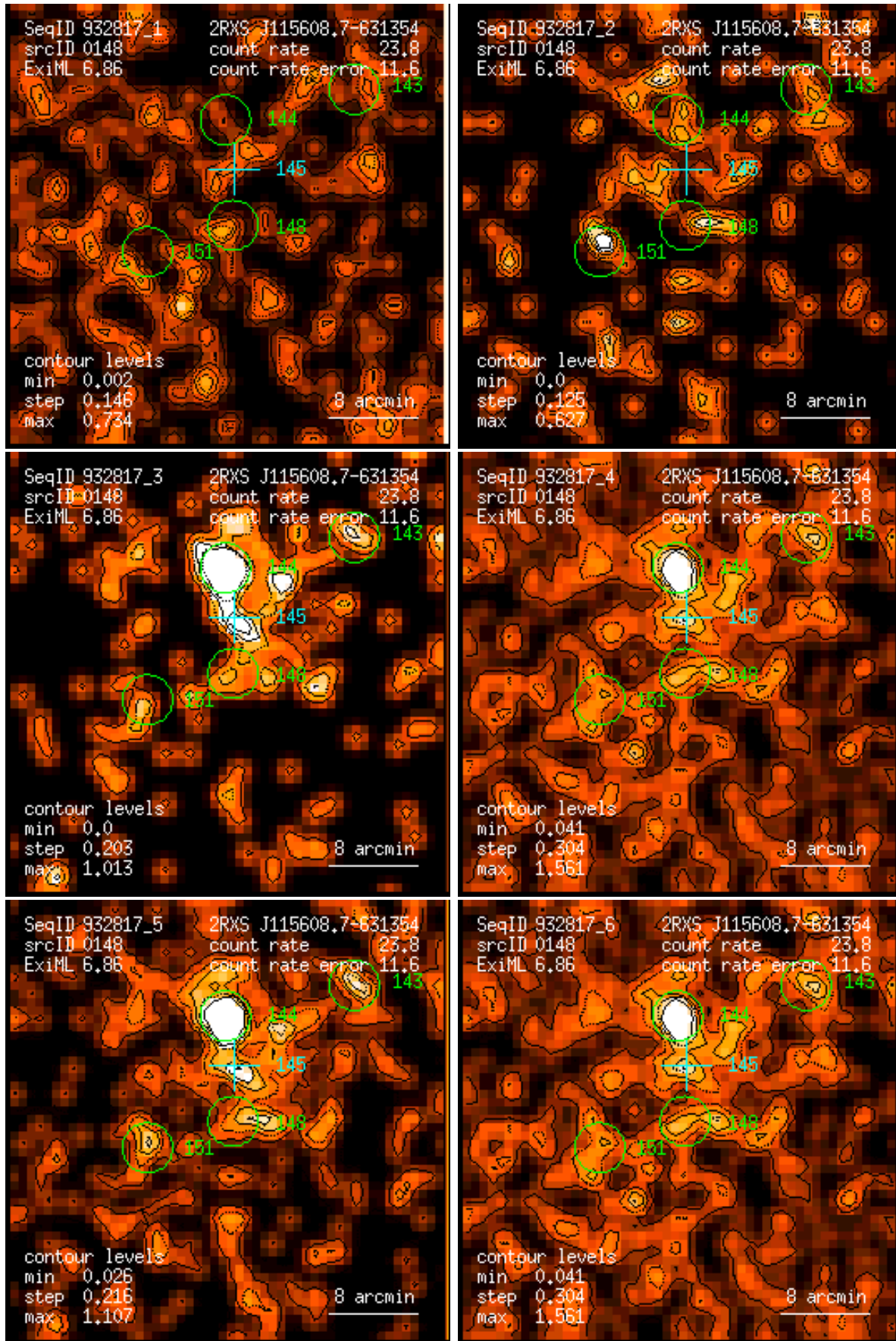
Figure 148: RASS 932817: detection 0148: band rate images, Gaussian filter: (1) PSPC channels 11 – 41, (2) 52 – 90, (3) 91 – 201, (4) 11 – 235, (5) 52 – 201, (6) 11 – 201. Broad band rates in counts/ks. Band rate contour levels in counts/ks/arcmin 2 .
