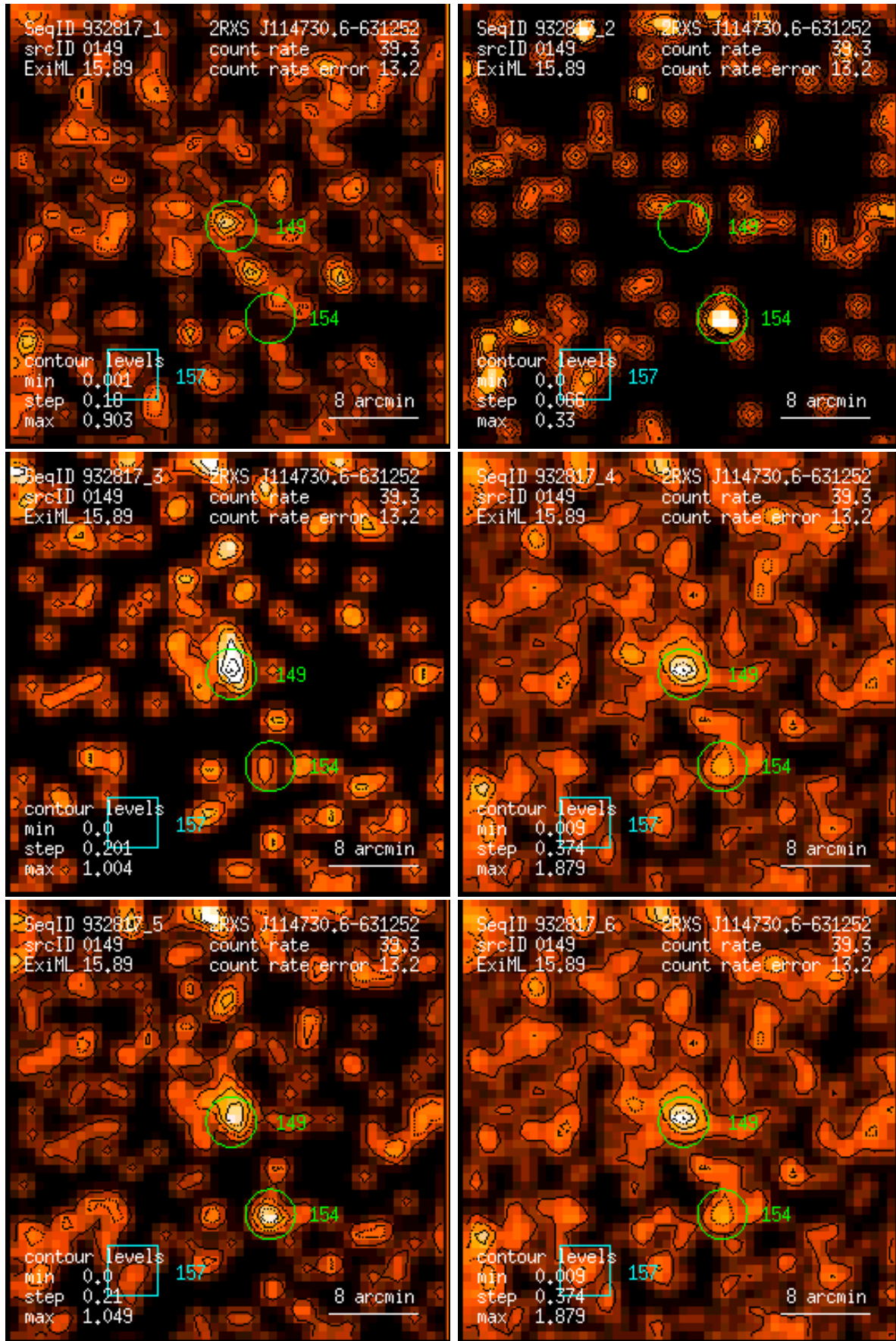
Figure 149: RASS 932817: detection 0149: band rate images, Gaussian filter: (1) PSPC channels 11 – 41, (2) 52 – 90, (3) 91 – 201, (4) 11 – 235, (5) 52 – 201, (6) 11 – 201. Broad band rates in counts/ks. Band rate contour levels in counts/ks/arcmin 2 .
