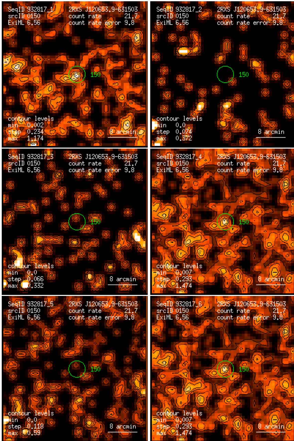
Figure 150: RASS 932817: detection 0150: band rate images, Gaussian filter: (1) PSPC channels 11 – 41, (2) 52 – 90, (3) 91 – 201, (4) 11 – 235, (5) 52 – 201, (6) 11 – 201. Broad band rates in counts/ks. Band rate contour levels in counts/ks/arcmin 2 .
