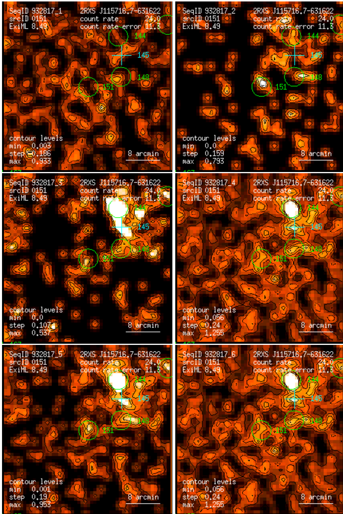
Figure 151: RASS 932817: detection 0151: band rate images, Gaussian filter: (1) PSPC channels 11 – 41, (2) 52 – 90, (3) 91 – 201, (4) 11 – 235, (5) 52 – 201, (6) 11 – 201. Broad band rates in counts/ks. Band rate contour levels in counts/ks/arcmin 2 .
