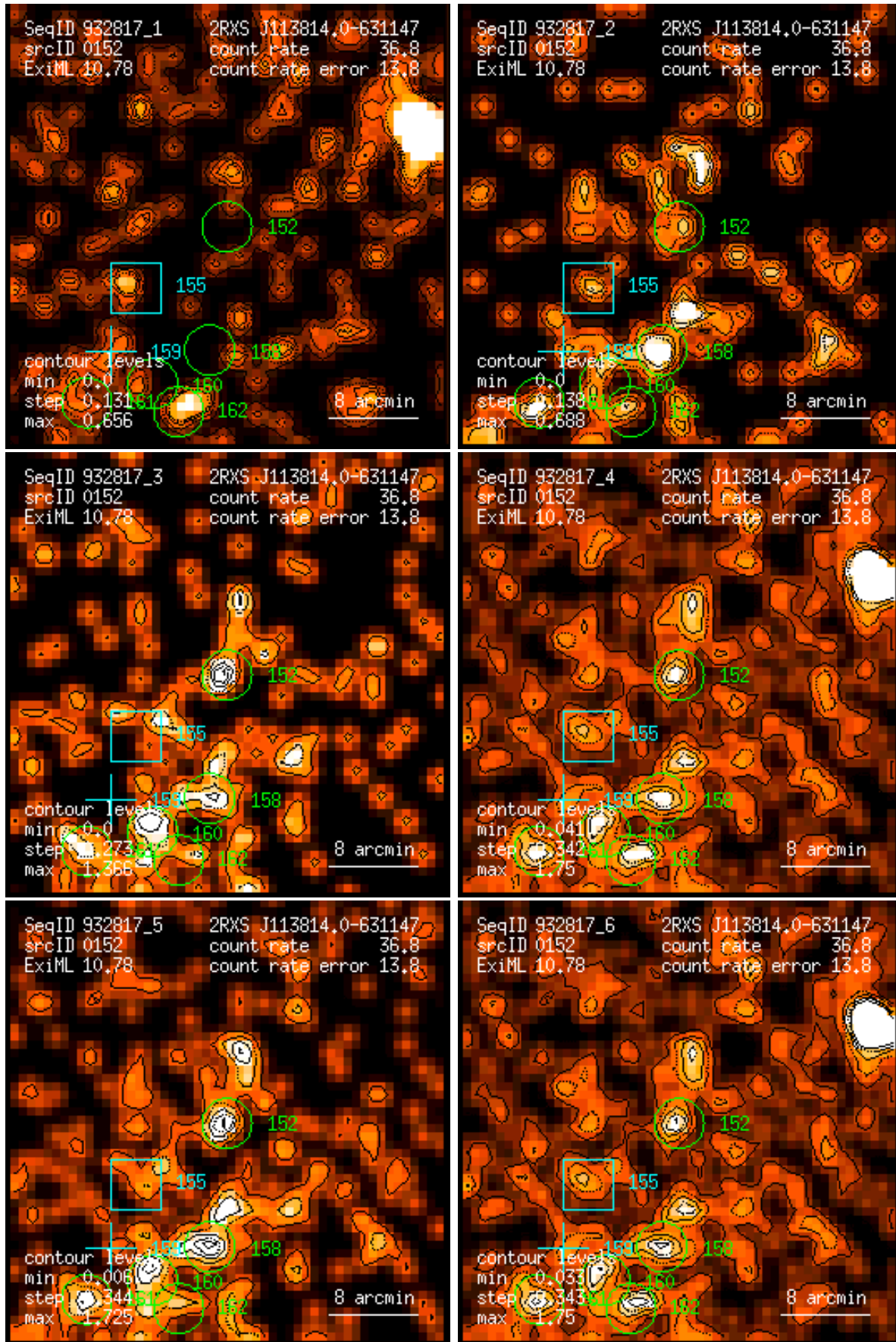
Figure 152: RASS 932817: detection 0152: band rate images, Gaussian filter: (1) PSPC channels 11 – 41, (2) 52 – 90, (3) 91 – 201, (4) 11 – 235, (5) 52 – 201, (6) 11 – 201. Broad band rates in counts/ks. Band rate contour levels in counts/ks/arcmin 2 .
