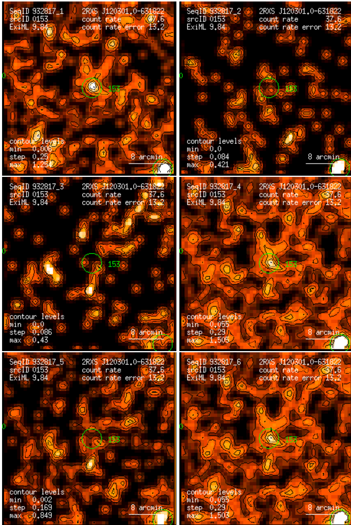
Figure 153: RASS 932817: detection 0153: band rate images, Gaussian filter: (1) PSPC channels 11 – 41, (2) 52 – 90, (3) 91 – 201, (4) 11 – 235, (5) 52 – 201, (6) 11 – 201. Broad band rates in counts/ks. Band rate contour levels in counts/ks/arcmin 2 .
